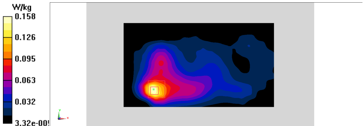
Fig.14 2450 MHz
