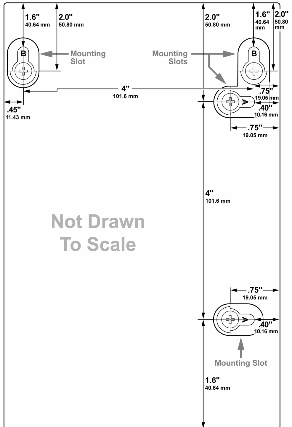
DPC2223 and EPC2223 Wall Mount Template
