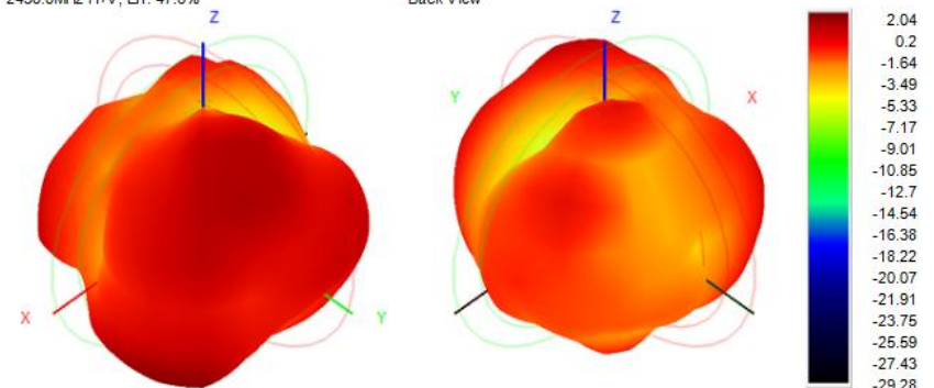
2450.0MHz H+V, Eff: 47.6%
