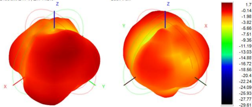
2500.0MHz H+V, Eff: 43.5%
