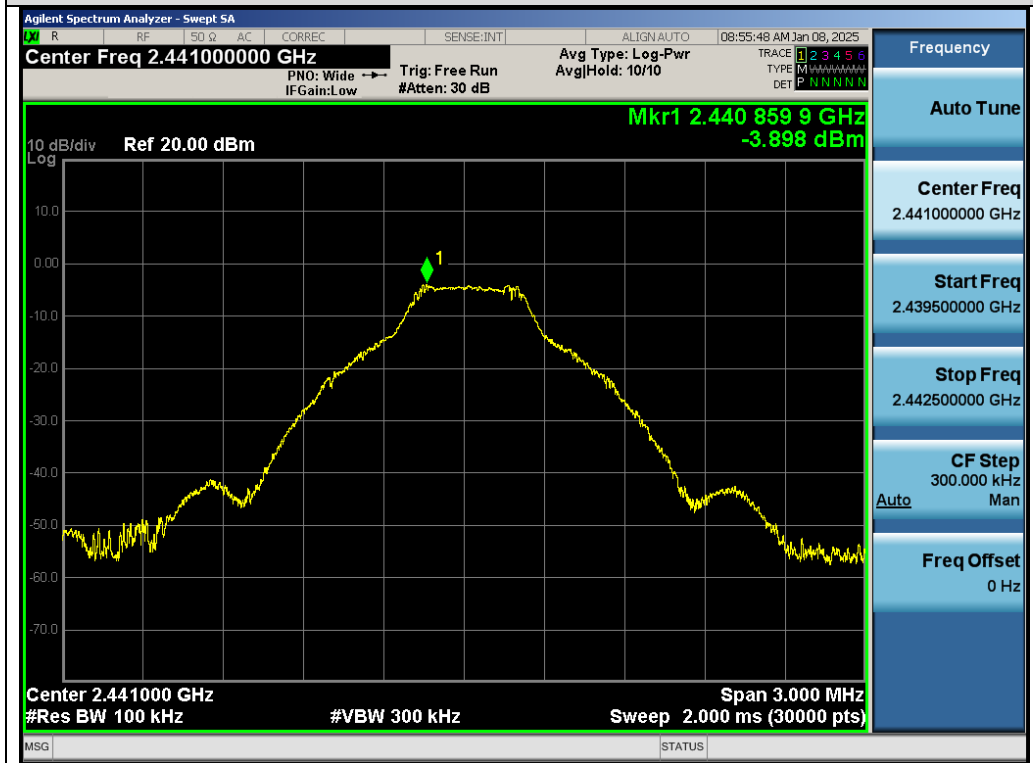
Test_Graph_GFSK_ANT1_2441_Reference Level
