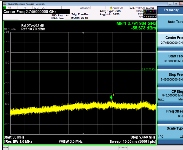
11N40SISO_Ant1_5510_5735~40000
