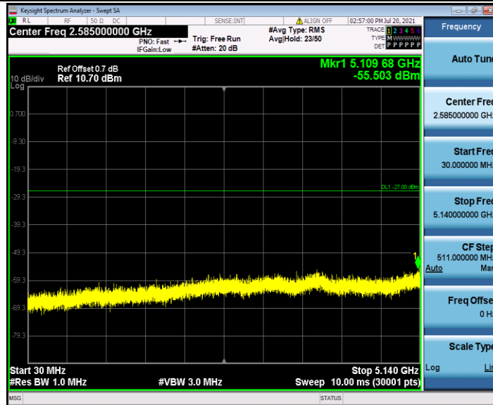
11N40SISO_Ant1_5310_5360~40000
