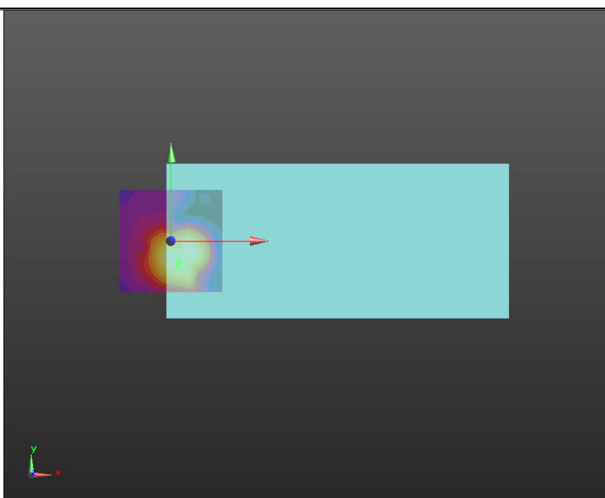
General Scans_LTE band5_T-Coil_HAC 3/z (axial) wideband at best S/N/ABM Freq Resp(x,y,z,f) Loc: 3.7, -12.3, 3.7 mm Diff: 0.18dB
