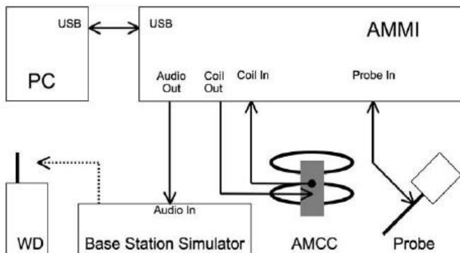
Test setup for WCDMA/VoLTE/VoWiFi CMRS service
