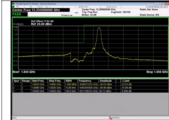
Band 2 1.4MHz/1850.7/Low 16QAM 1@5
