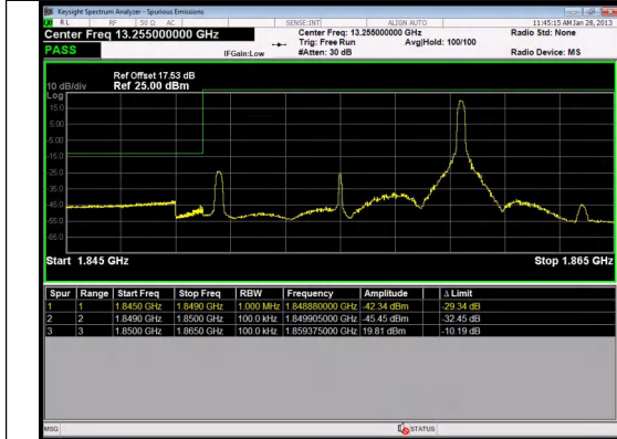
Band 2 10MHz/1855.0/Low 16QAM 1@49
