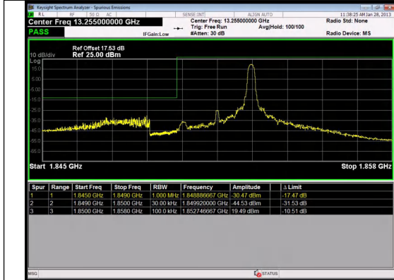
Band 2 3MHz/1851.5/Low 16QAM 1@14
