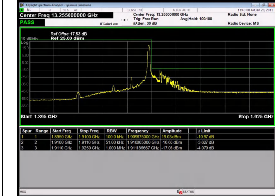
Band 2 5MHz/1907.5/High 16QAM 1@24
