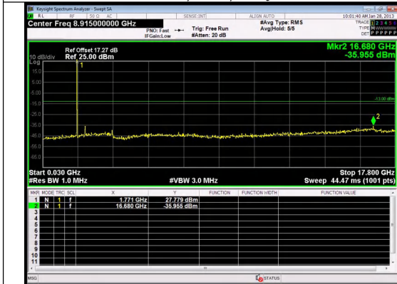
30.0MHz-17800.0MHz Band 66 10MHz/1775.0/High QPSK 1@0
