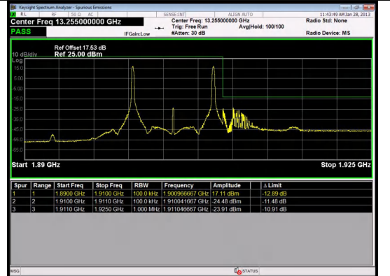
Band 2 10MHz/1905.0/High 16QAM 50@0
