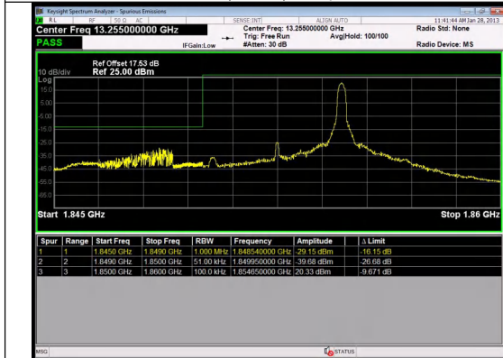
Band 2 5MHz/1852.5/Low 16QAM 1@24
