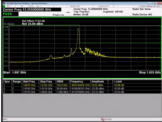
Band 2 3MHz/1908.5/High 16QAM 1@14
