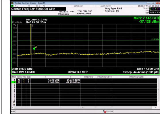
30.0MHz-17800.0MHz Band 66 10MHz/1745.0/Mid QPSK 1@0
