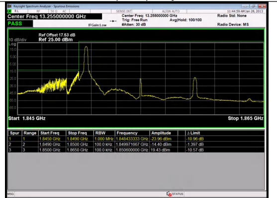
Band 2 10MHz/1855.0/Low 16QAM 1@0
