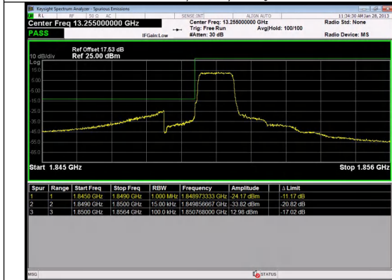
Band 2 1.4MHz/1850.7/Low QPSK 6@0
