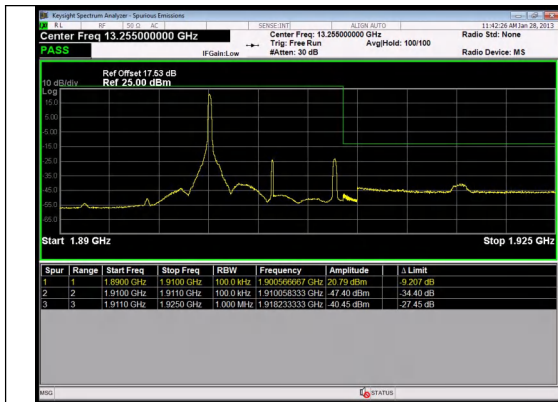
Band 2 10MHz/1905.0/High QPSK 1@0
