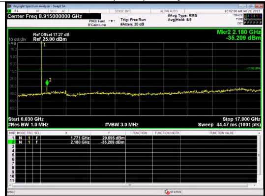
30.0MHz-17800.0MHz Band 66 10MHz/1775.0/High 16QAM 1@0
