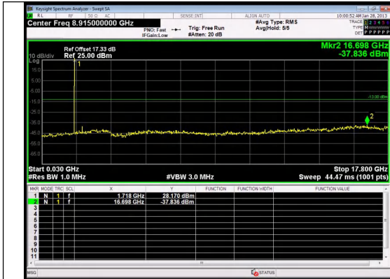
30.0MHz-17800.0MHz Band 66 5MHz/1712.5/Low QPSK 1@0
