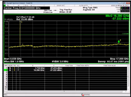
30.0MHz-17800.0MHz Band 66 5MHz/1712.5/Low 16QAM 1@0
