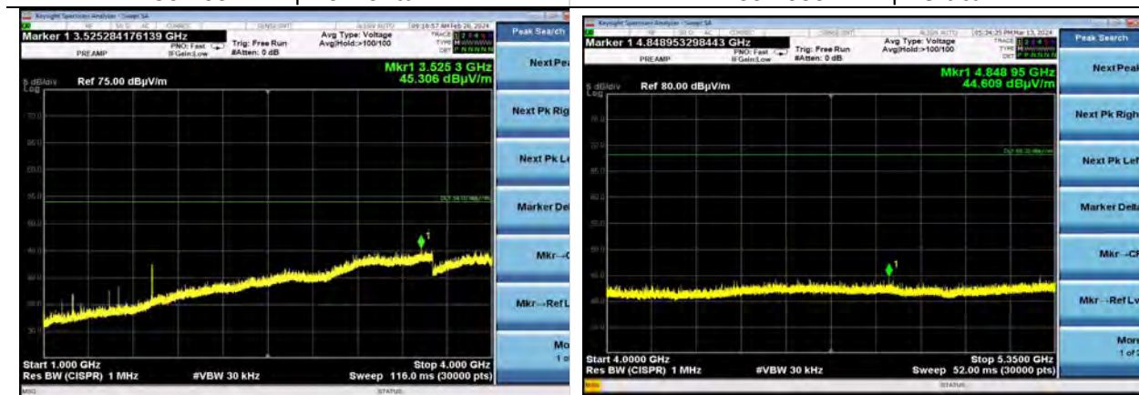
802.11a | Channel 100 | 6 Mbps | Y Plane 1000-4000 MHz | Horizontal
