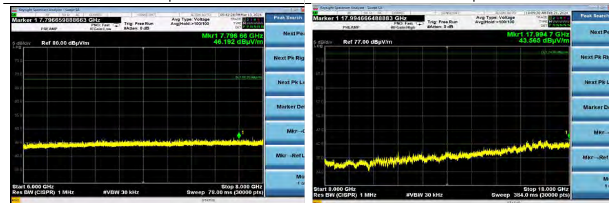
802.11a | Channel 100 | 6 Mbps | X Plane 6000-8000 MHz | Vertical
