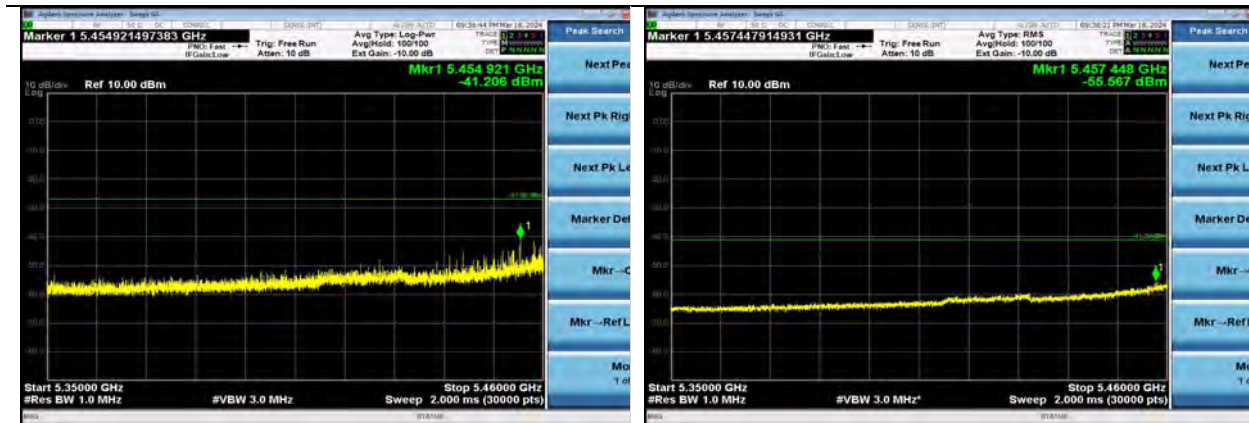
802.11ax20 | Channel 100 | MCS0 | Peak
