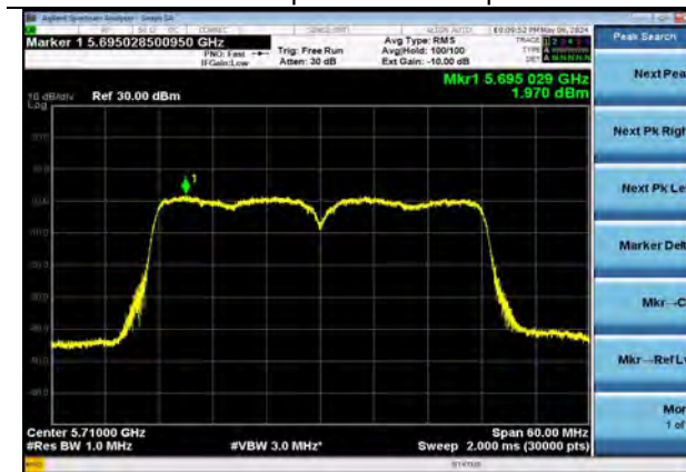
802.11n40 | Channel 142 | MCS7
