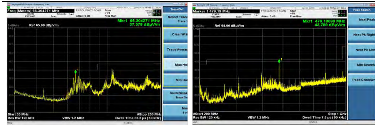
802.11a | Channel 120 | 6 Mbps | Y Plane 30-200 MHz | Horizontal
