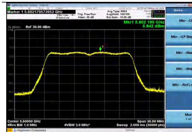
802.11a | Channel 120 | 54 Mbps
