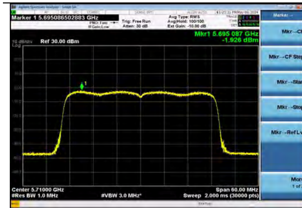
802.11ax40 | Channel 142 | MCS0
