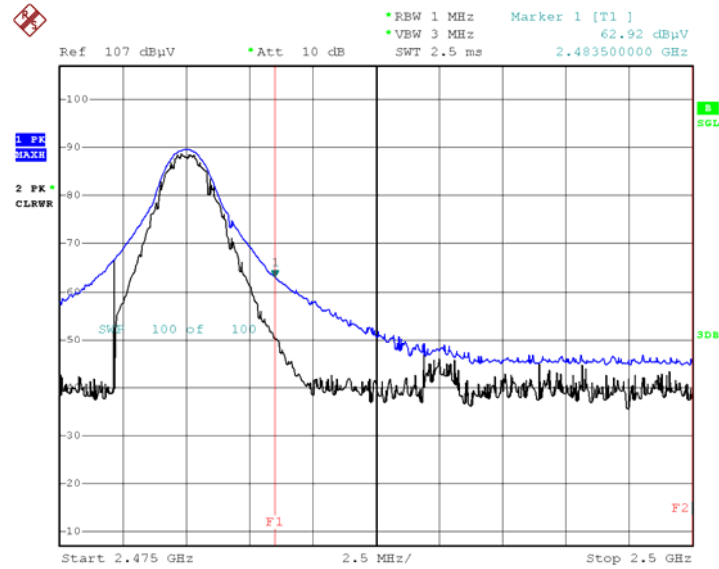
Radiated Restricted Band Edges plot – (8DPSK, Ch.78, X-V)
