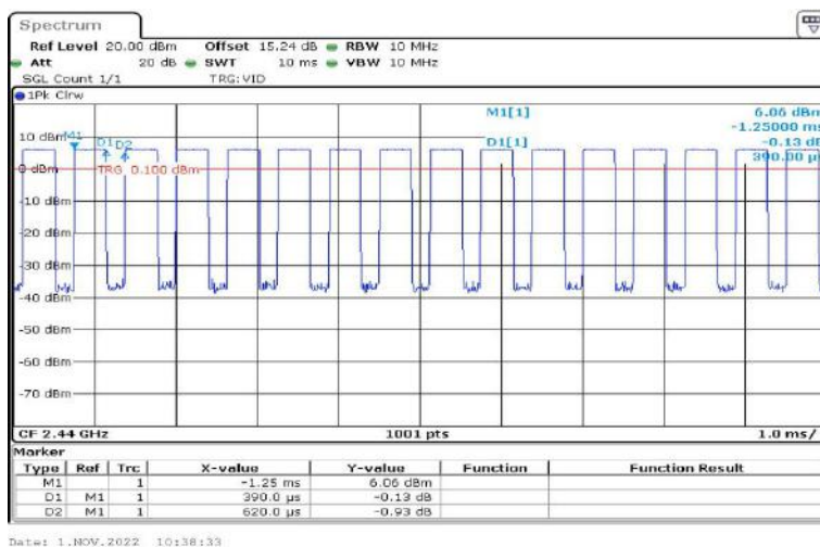
BLE_2M_Ant1_2440
