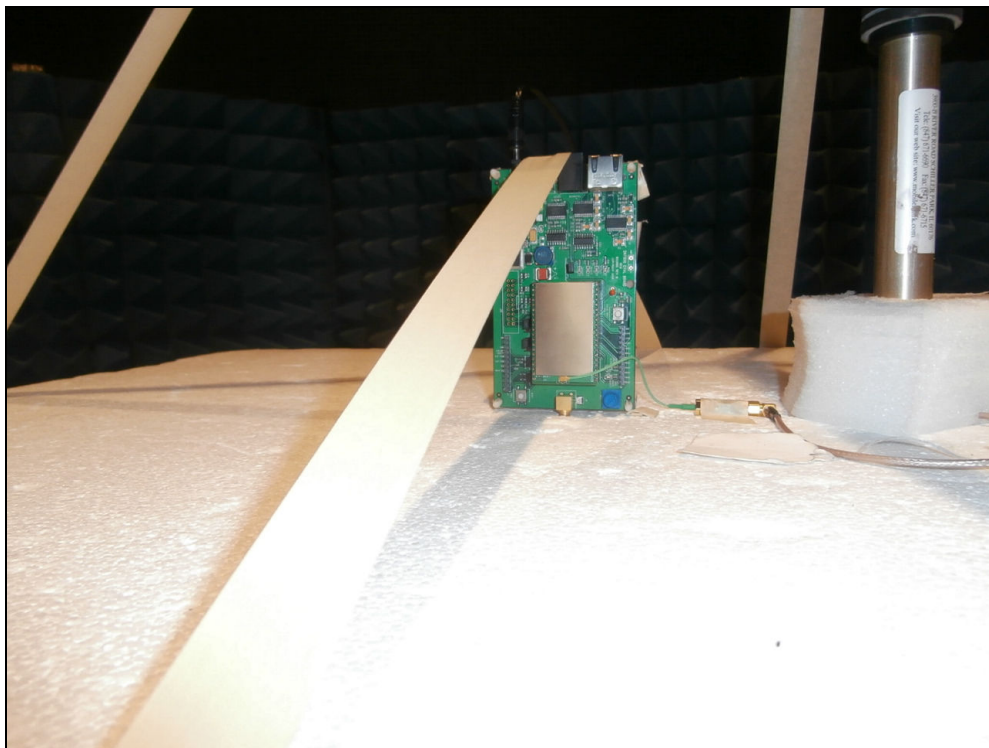
Figure 2: Radiated Emissions – YPOS – Dipole Antenna
