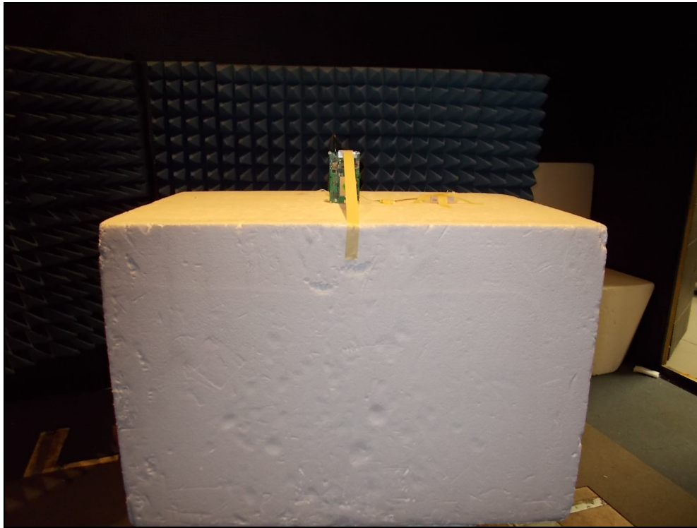
Figure 5: Radiated Emissions – YPOS – Patch Antenna
