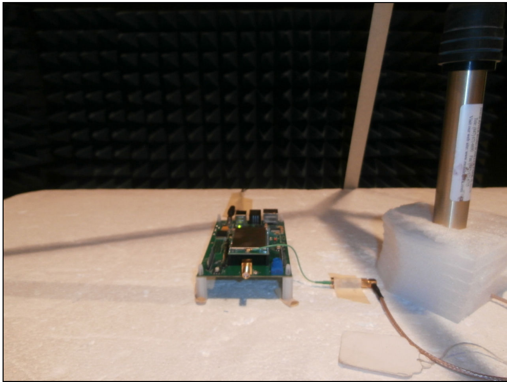
Figure 3: Radiated Emissions – ZPOS – Dipole Antenna
