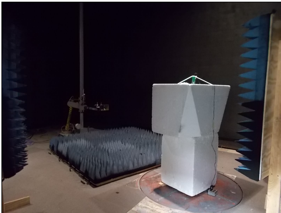
Figure 6: Radiated Emissions – YPOS – Patch Antenna
