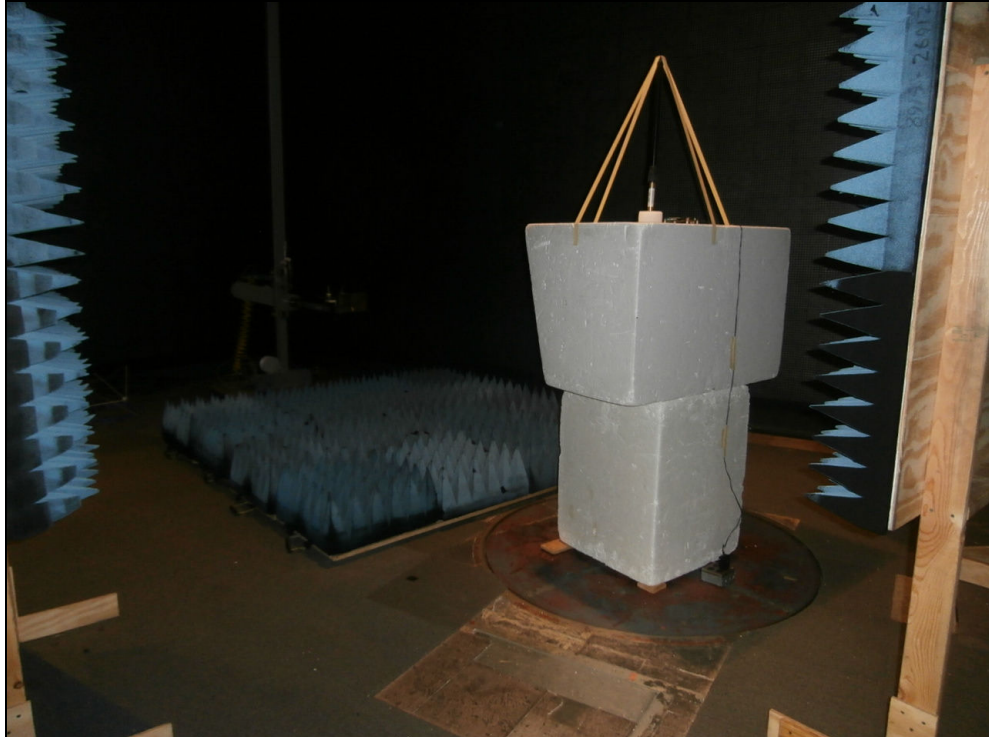
Figure 4: Radiated Emissions – ZPOS – Dipole Antenna
