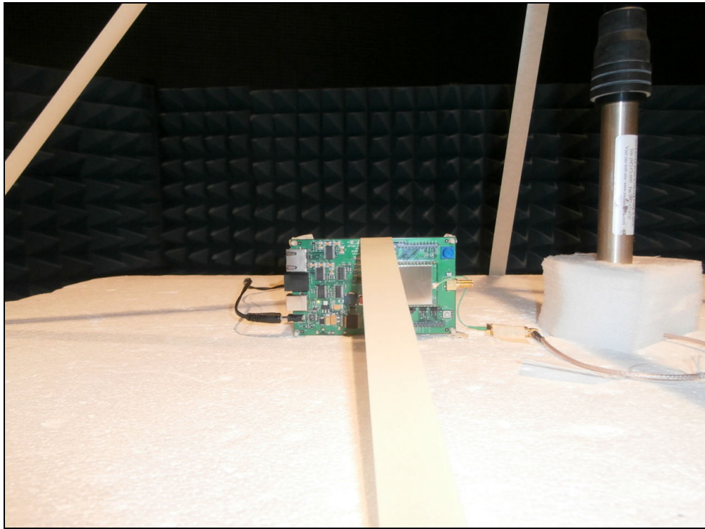
Figure 1: Radiated Emissions – XPOS – Dipole Antenna
