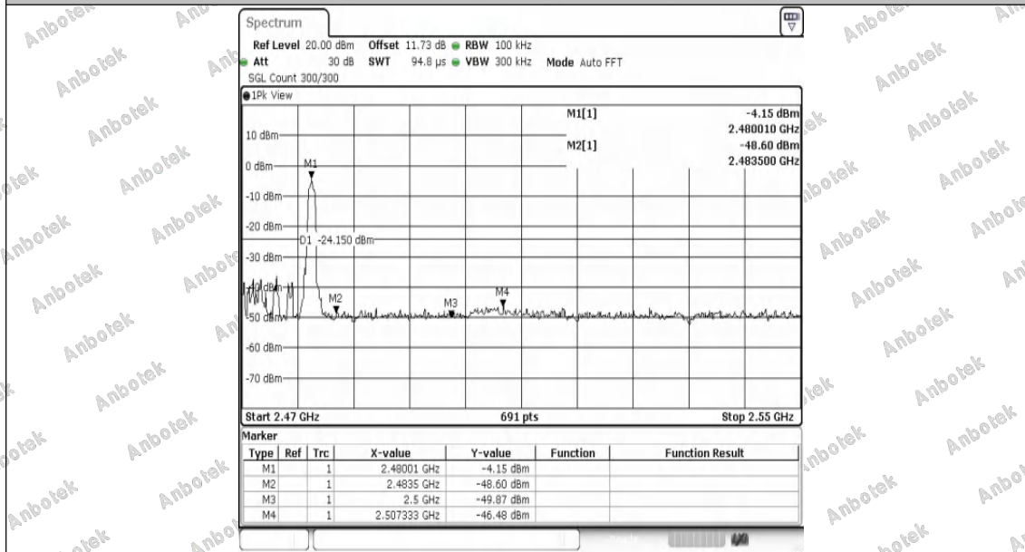
3DH5-Ant1-2480-PASS
