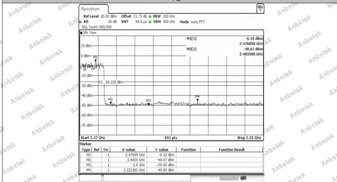
2DH5-Ant1-Hop_2480-PASS
