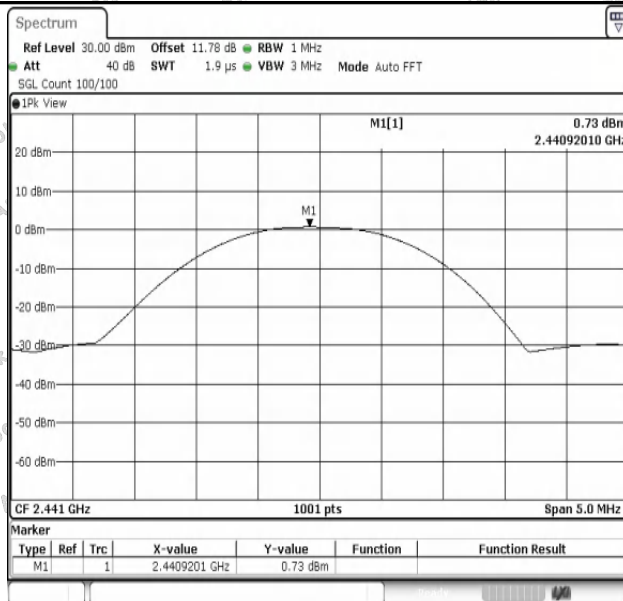
DH5-Ant1-2441-PASS
