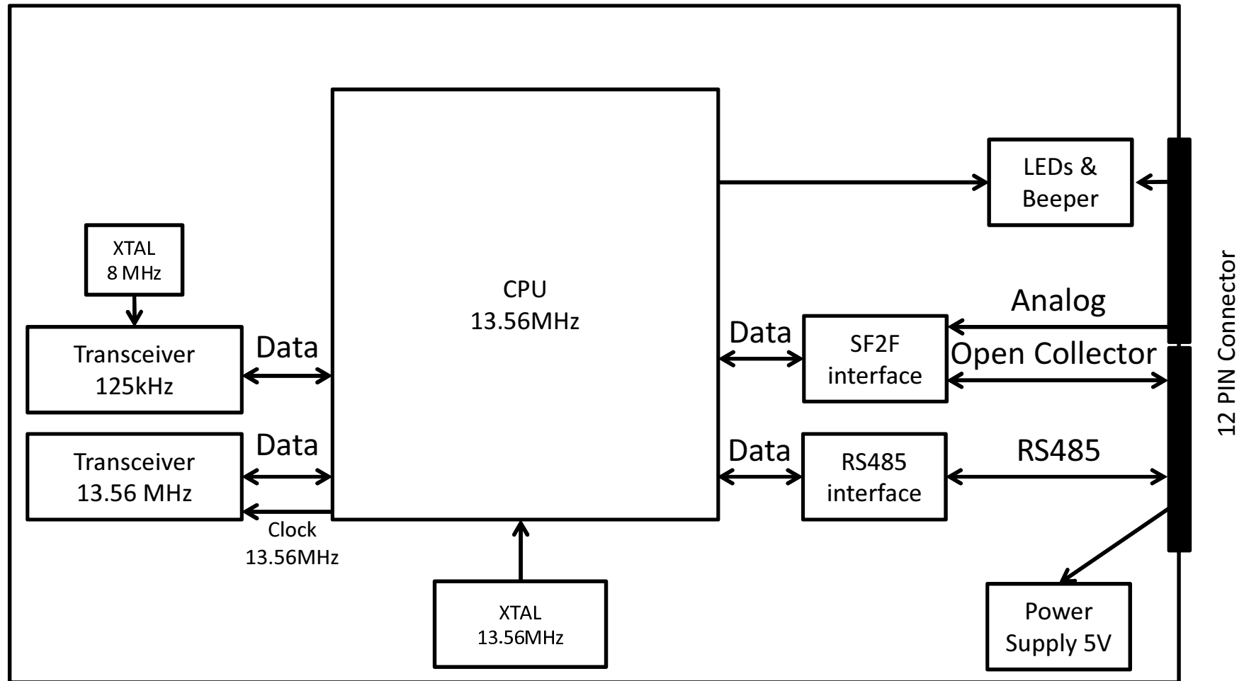
Block Diagram PRD5/2 HID SF2F
