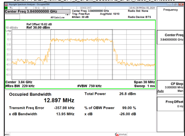
Band77-Part27_15MHz_DFT_s_OFDM_SCS30kHz_BPSK_RB36_0_CH656000
