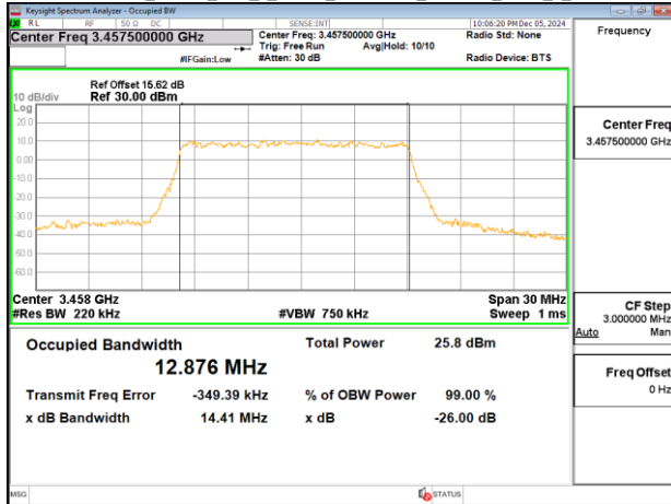
Band77-Part27_15MHz_DFT_s_OFDM_SCS30kHz_256QAM_RB36_0_CH633334
