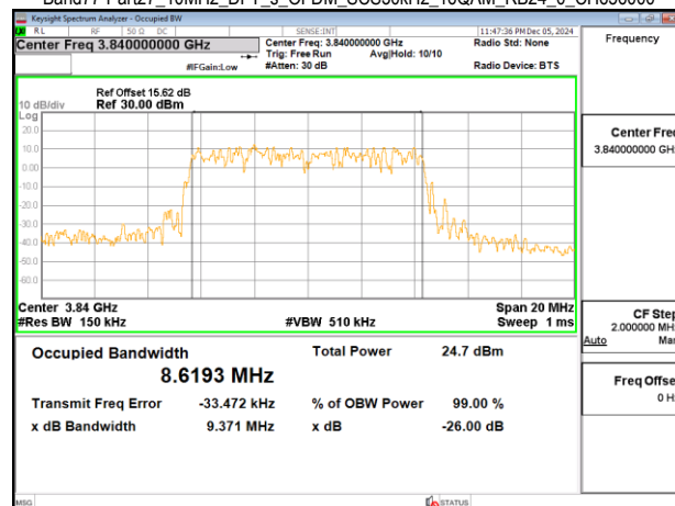
Band77-Part27_10MHz_DFT_s_OFDM_SCS30kHz_16QAM_RB24_0_CH656000
