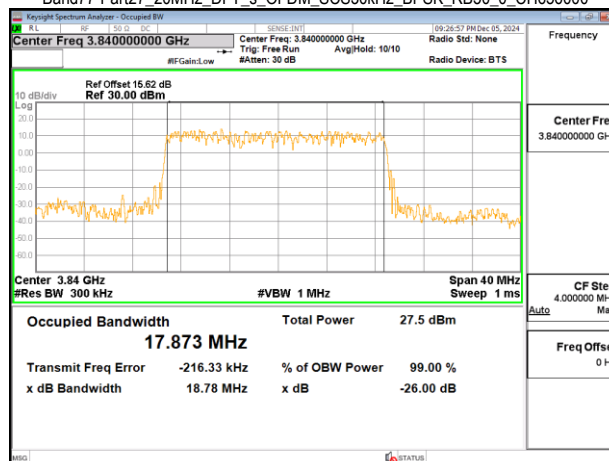
Band77-Part27_20MHz_DFT_s_OFDM_SCS30kHz_BPSK_RB50_0_CH656000
