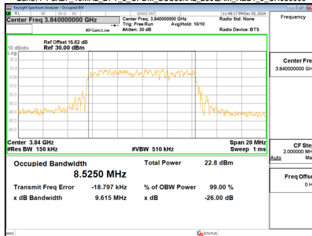
Band77-Part27_10MHz_DFT_s_OFDM_SCS30kHz_256QAM_RB24_0_CH656000
