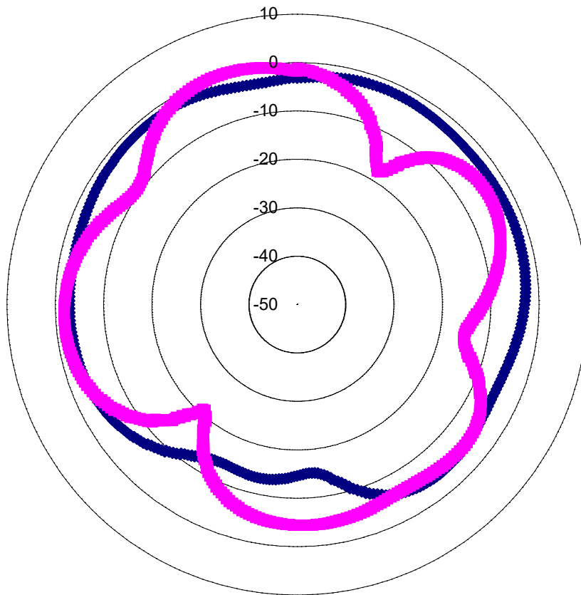
CS6529 BS ANT1 Radiation Pattern_XY Plane
