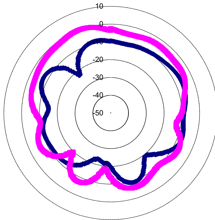
CS6529 BS BT Radiation Pattern_XY Plane
