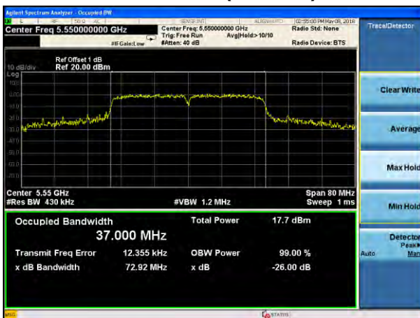
Channel 110 (5550MHz)
