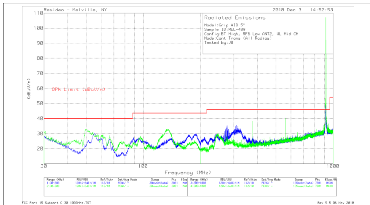
30-1000MHz – Plot
