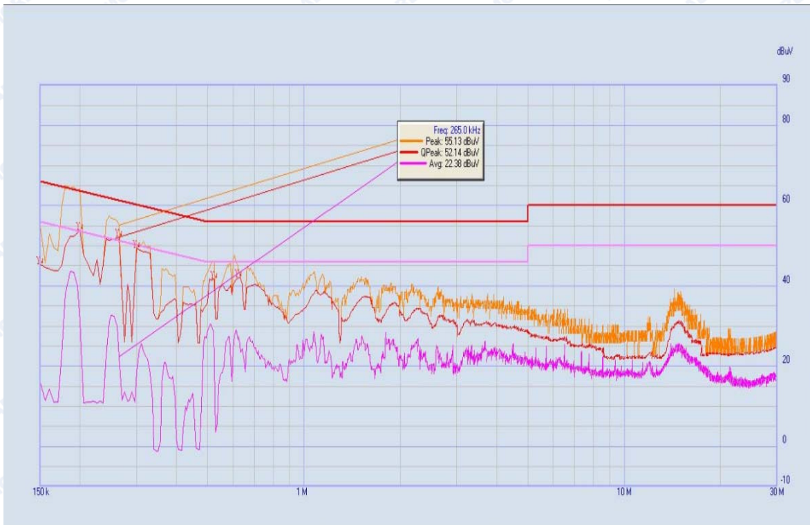
(Plot A: Data transmission mode, L Phase)
