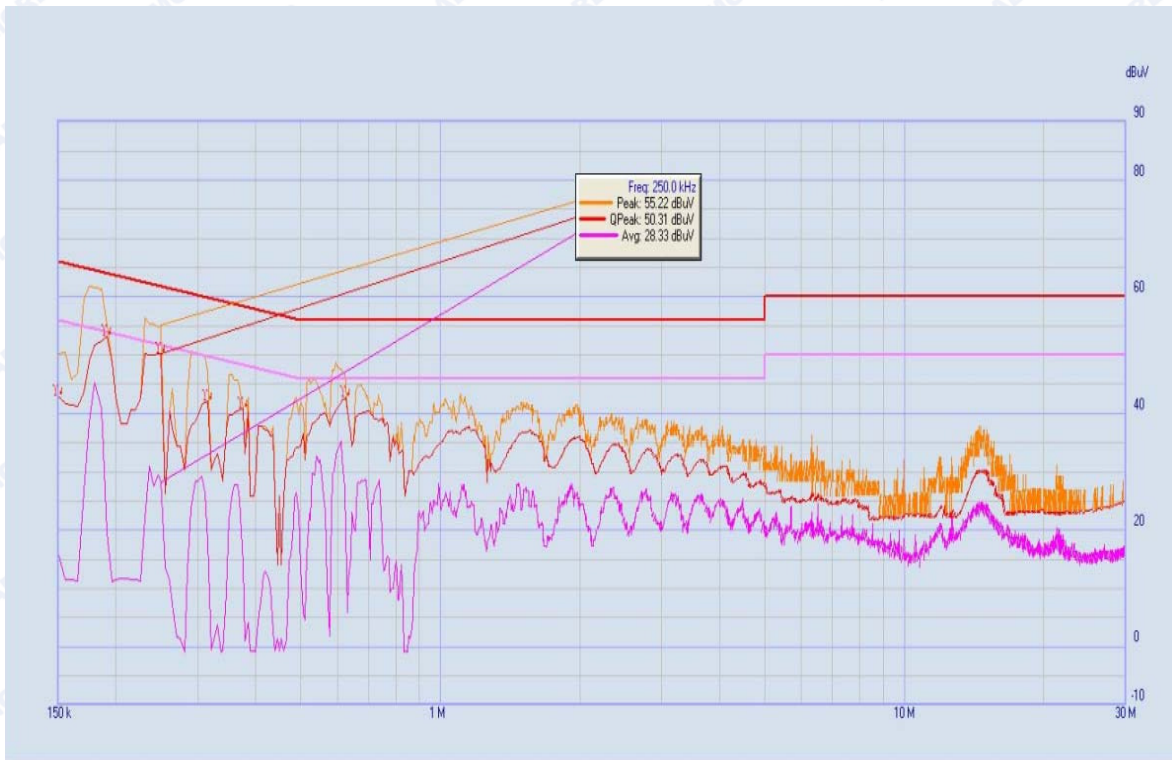
(Plot B: Data transmission mode, N Phase)
