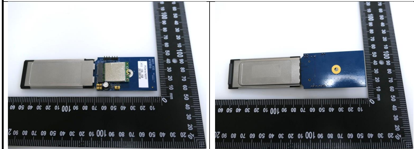
PCB
