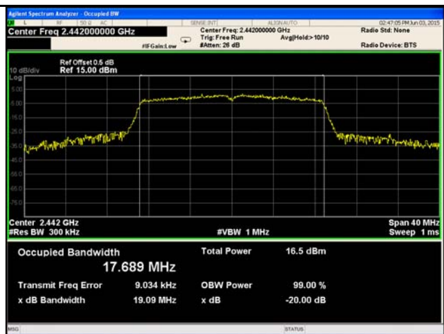
802.11n20 20dB Bandwidth - Mid CH 2442
