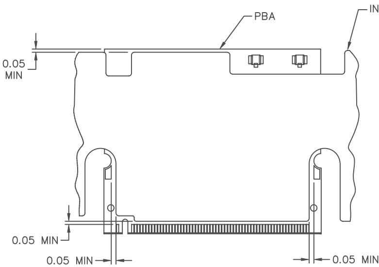
PRIMARY SIDE INSULATION PLACEMENT STEP 1
