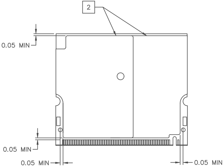
SECONDARY SIDE INSULATION PLACEMENT STEP 3
