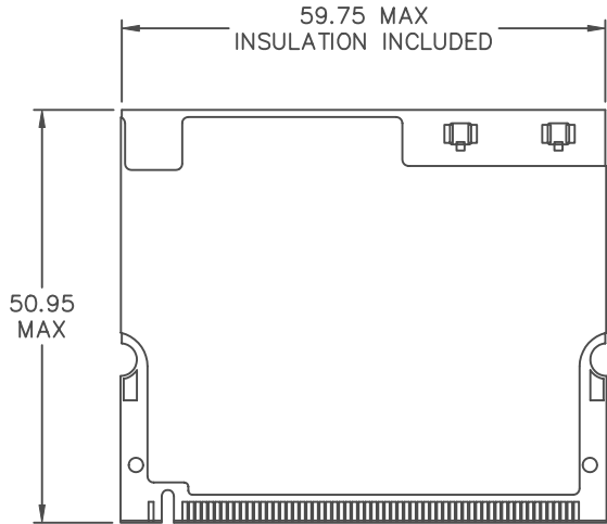
PRIMARY SIDE FINISHED ASSEMBLY
