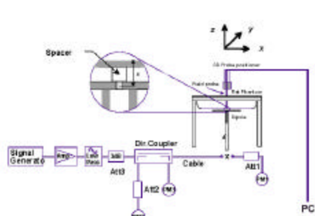
Figure 13.1 Dipole Validation Test Setup
