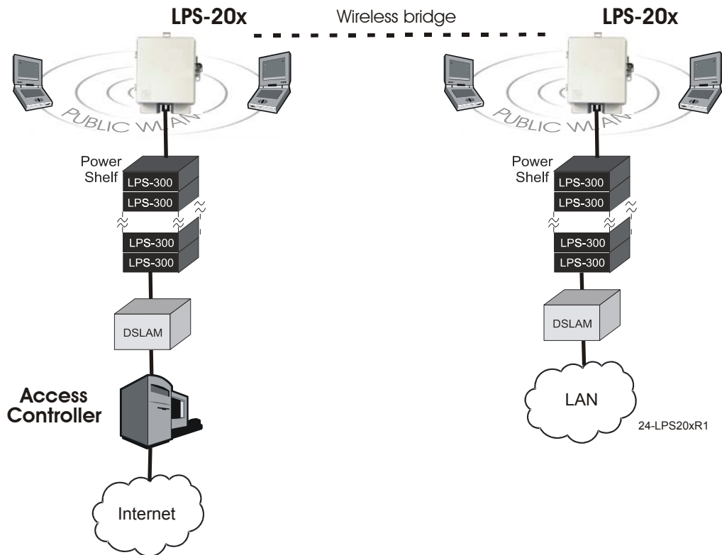
Figure 22. Wireless Bridging
