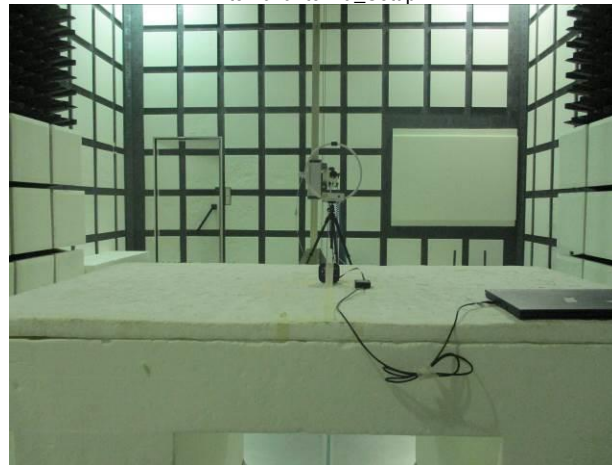
FCC_15_247+IC_RSS_247_902~928MHz_LoRa_Radiated_ External antenna_Setup
