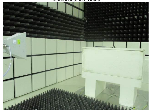
FCC_15_247+IC_RSS_247_902~928MHz_FSK_Radiated_ Internal antenna_Setup
