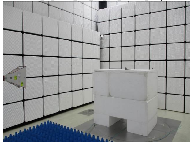
FCC_15_247+IC_RSS_247_BLE_Radiated_Setup
