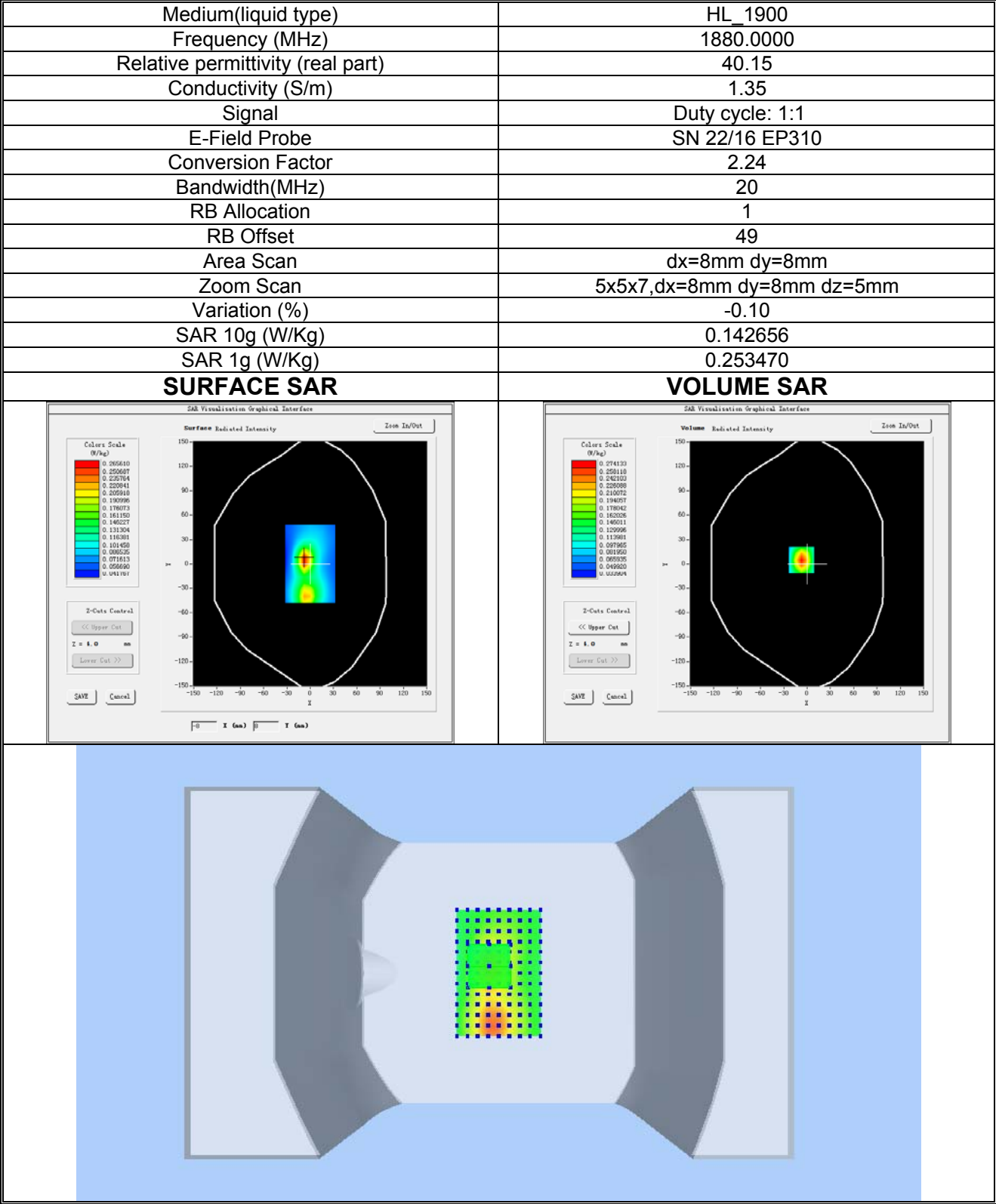
Plot 12:LTE BAND 2, Middle channel (Body-worn /Hotspot, Bottom Edge) Product Description:Smart Phone Test Date: 2023-05-12
