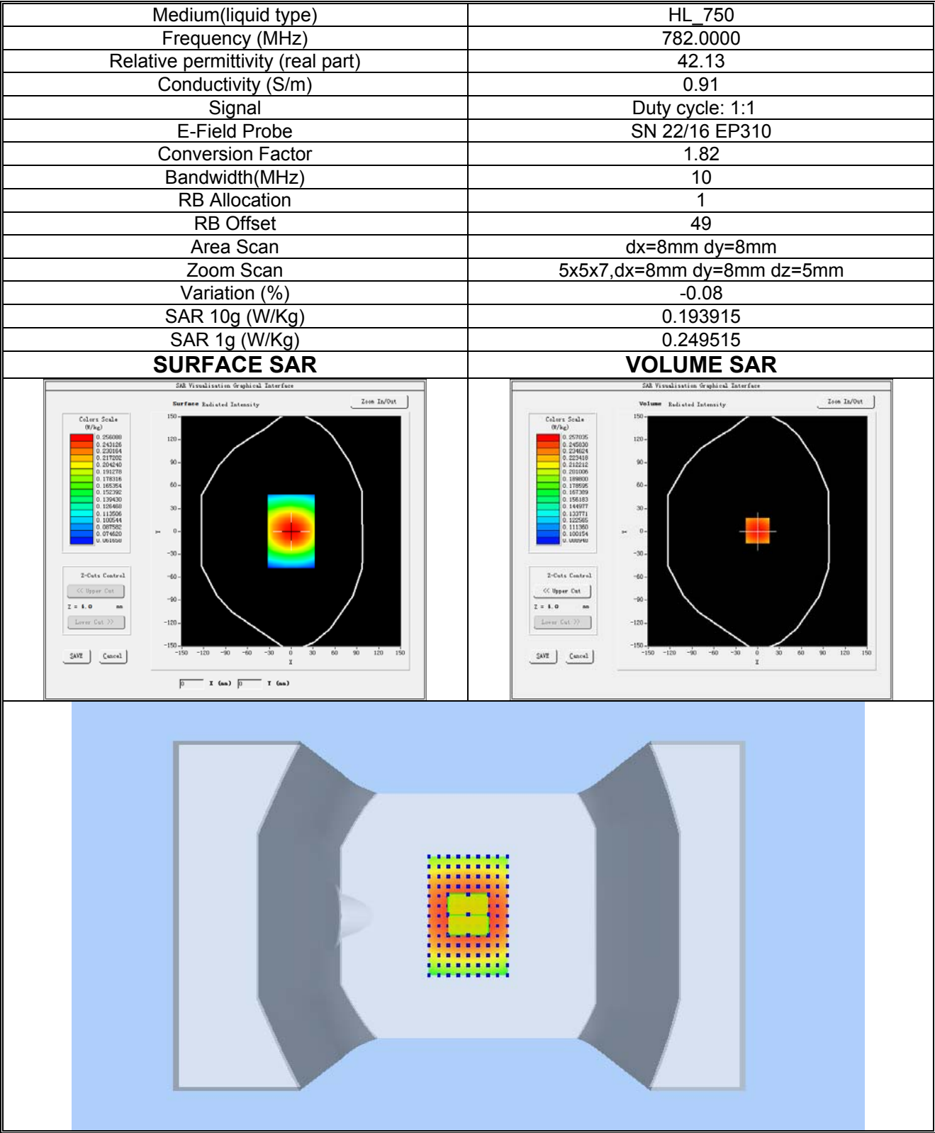
Plot 22: LTE BAND 13, Middle channel (Body-worn/ Hotspot, Back Side) Product Description: Smart Phone Test Date: 2023-05-16
