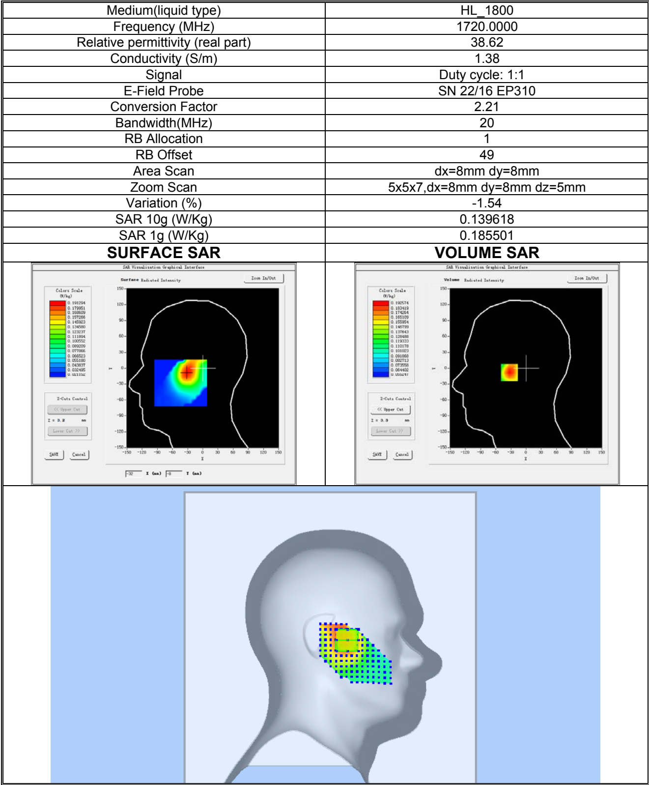
Plot 13:LTE BAND 4, Low channel (Left Head Cheek) Product Description: Smart Phone Test Date: 2023-05-11
