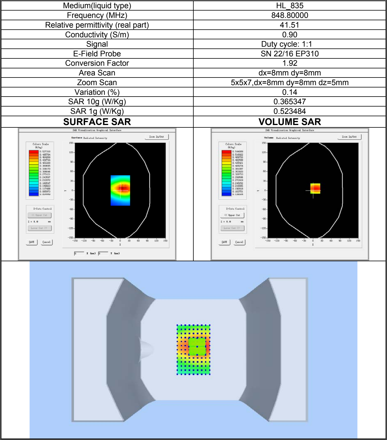
Plot 2: GPRS850MHz, High channel (Body-worn /Hotspot, Right Edge) Product Description:Smart Phone Test Date: 2023-05-18
