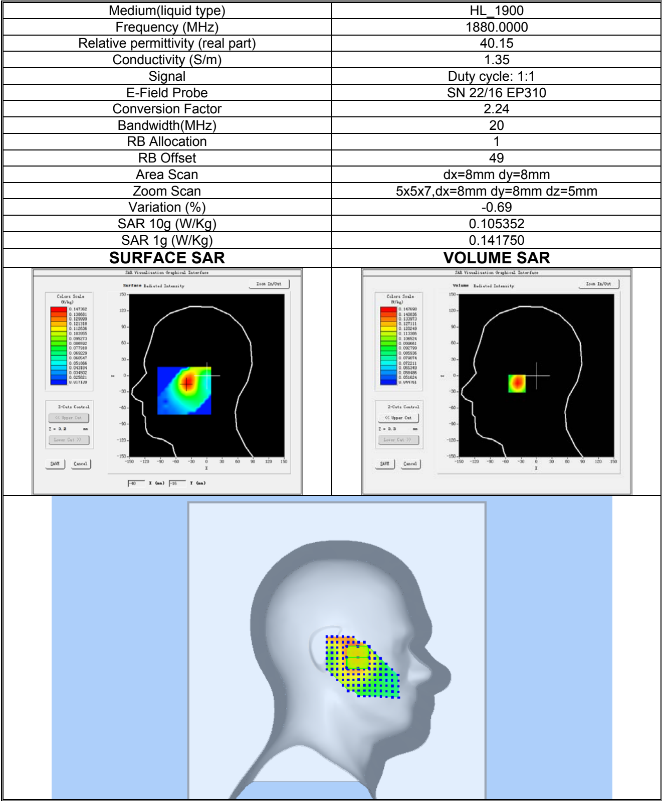
Plot 11:LTE BAND 2, Middle channel (Left Head Cheek) Product Description:Smart Phone Test Date: 2023-05-11
