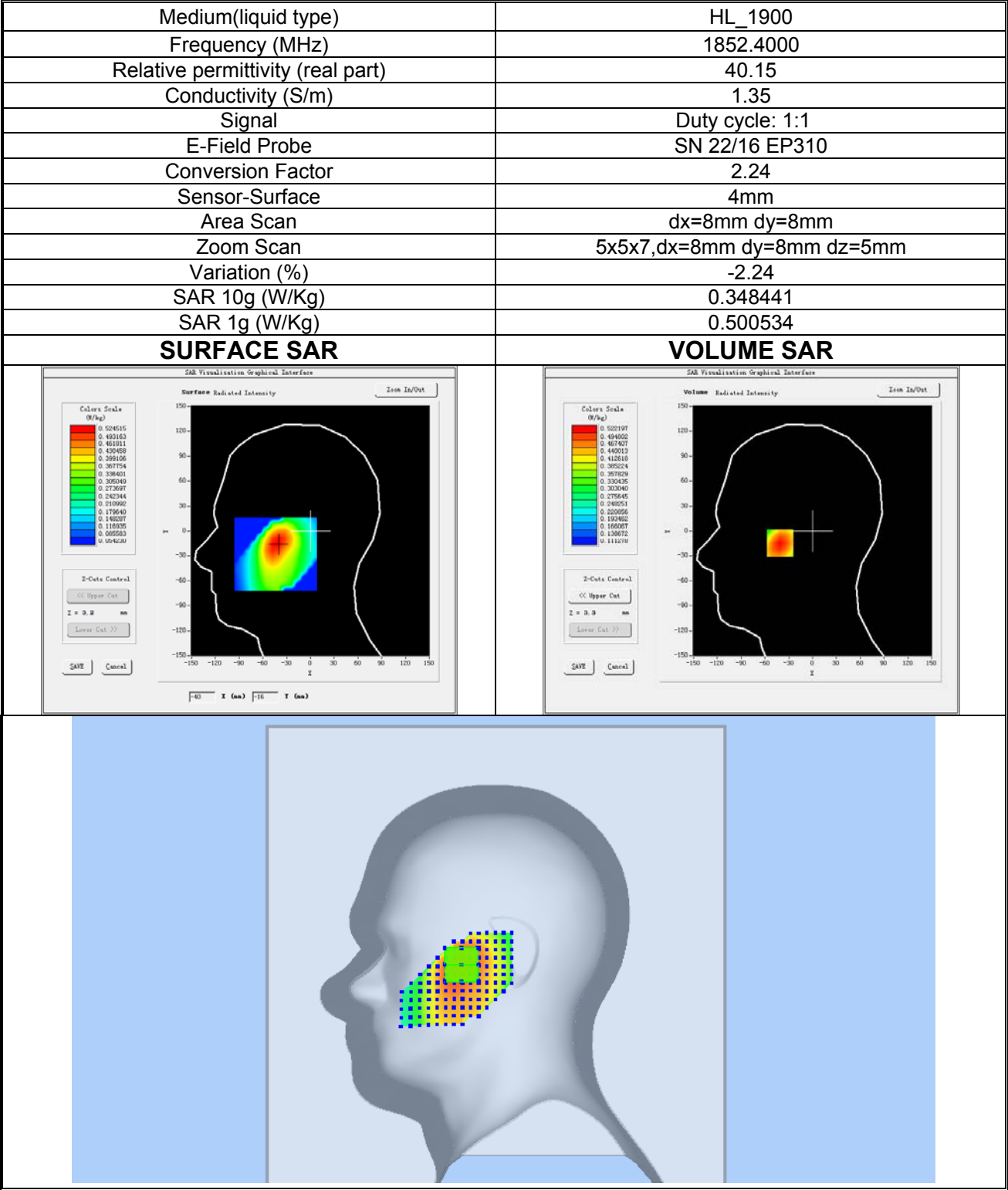
Plot 5: WCDMA BAND II, Low channel (Right Head Cheek) Product Description: Smart Phone Test Date: 2023-05-15
