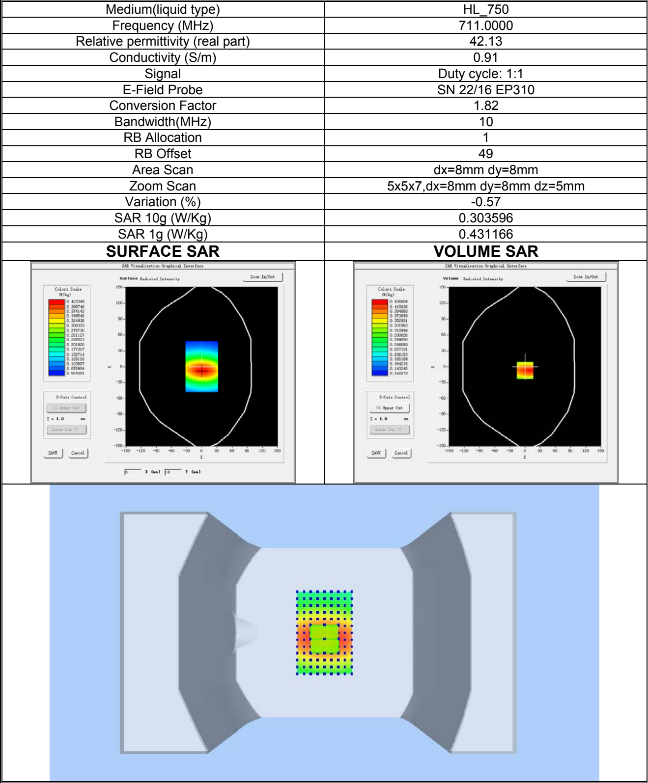
Plot 20: LTE BAND 12, High channel (Body-worn/ Hotspot, Right Edge) Product Description: Smart Phone Test Date: 2023-05-16
