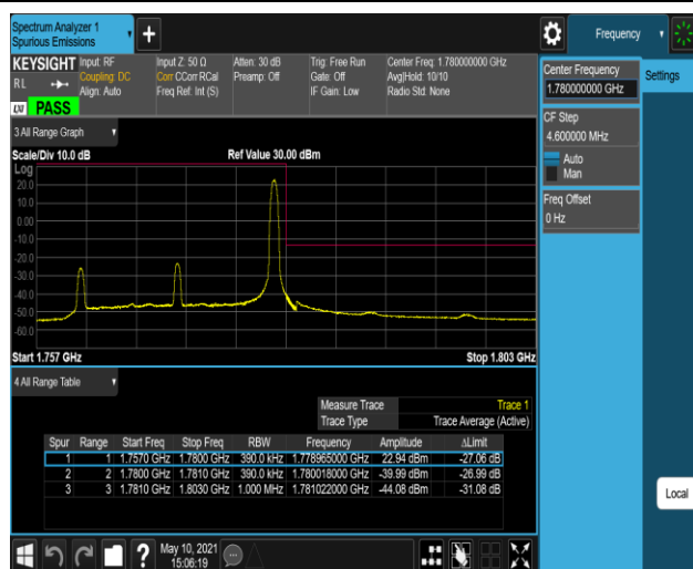
Band66-20MHz-16QAM-132572-1RB#99
