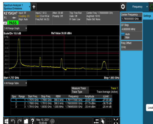
Band66-20MHz-16QAM-132572-100RB#0
