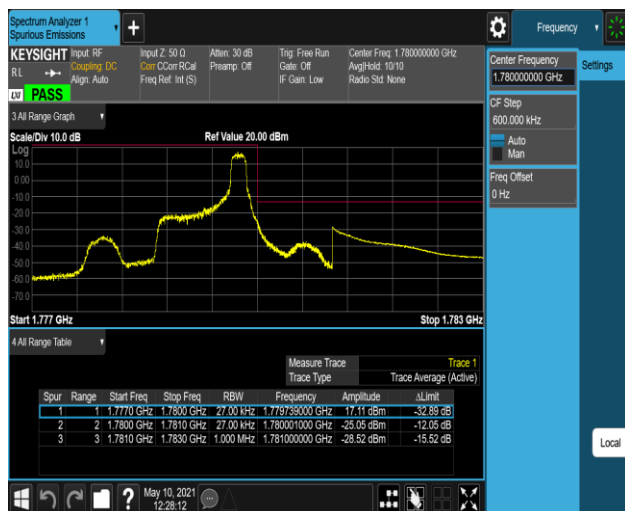
Band66-1.4MHz-QPSK-132665-1RB#5
