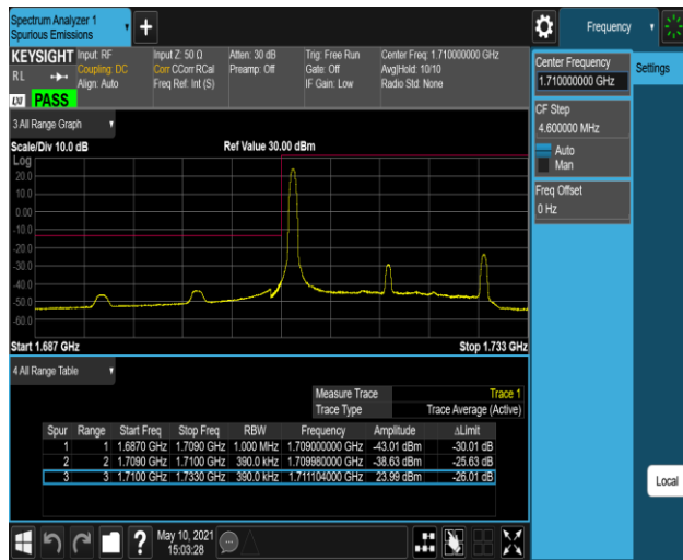
Band66-20MHz-QPSK-132072-100RB#0
