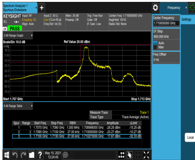
Band66-1.4MHz-QPSK-131979-6RB#0
