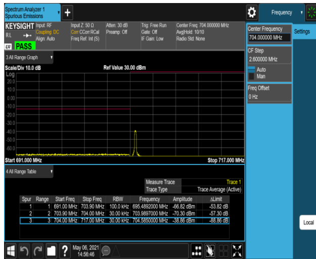
Band17-10MHz-QPSK-23780-50RB#0
