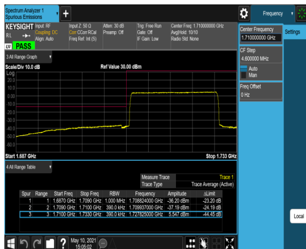
Band66-20MHz-16QAM-132572-1RB#99
