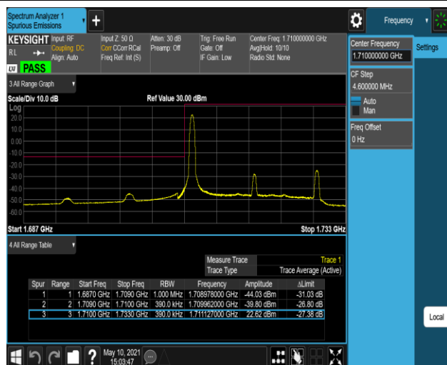
Band66-20MHz-16QAM-132072-100RB#0
