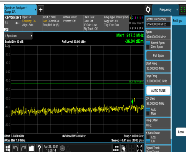
Band2-20MHz-16QAM-19100-1RB#0-Range1:30~1
