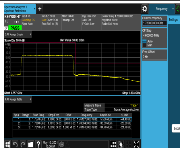
Band66-20MHz-16QAM-132572-100RB#0
