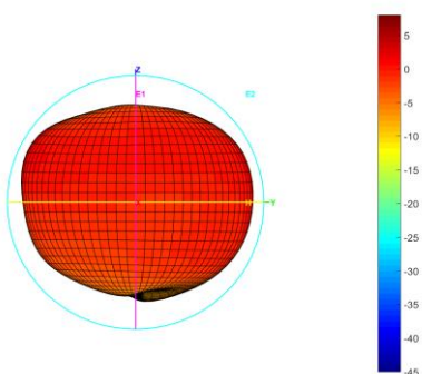
Total_3D_E2_2.45GHz
