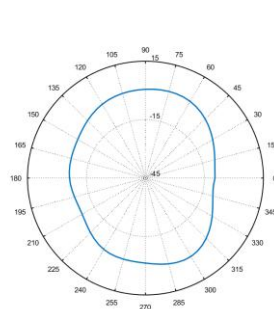
Total_Polar_E2_2.45GHz
