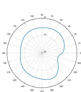
Total_Polar_E1_2.45GHz
