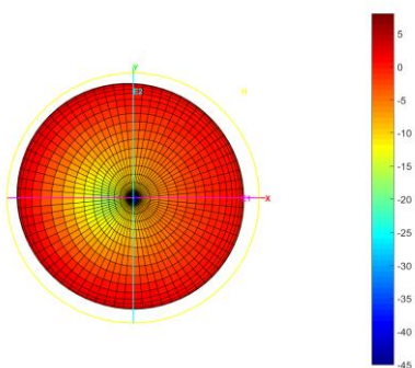
Total_3D_H_2.45GHz
