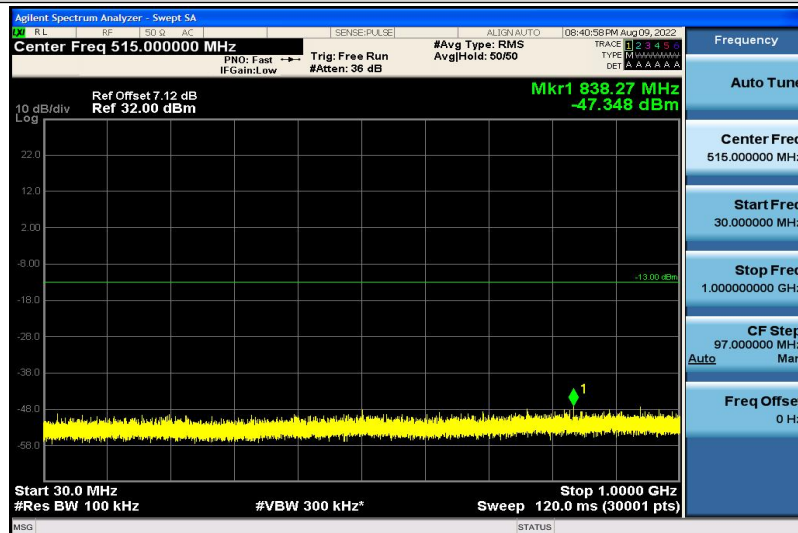
Band4-15MHz-16QAM-20025-1RB#0-30~1000MHz
