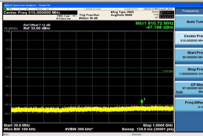
Band4-5MHz-QPSK-19975-1RB#0-30~1000MHz
