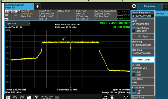
Channel 11 (2462MHz)
