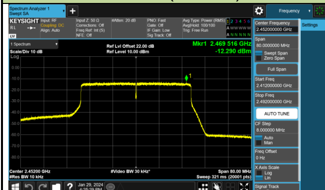
Channel 09 (2452MHz)
