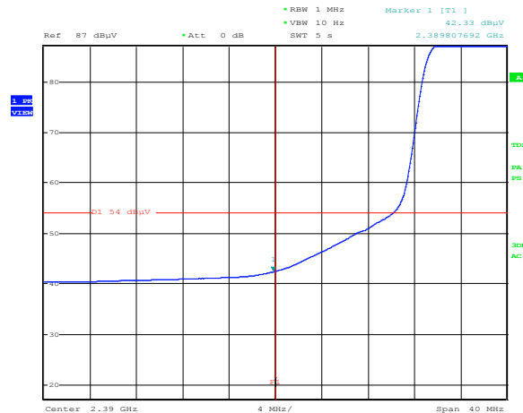
Figure 8.4-35: Radiated spurious emissions Lower band edge for 802.11n HT20, (TX 2412 MHz) – Average
