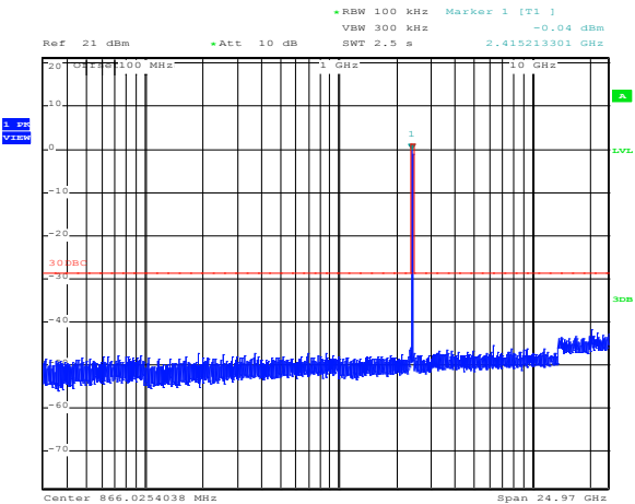
Figure 8.4-2: Conducted spurious emissions for 802.11g (TX 2412 MHz)
