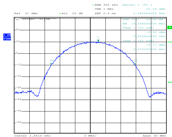
Figure 8.2-10: 20 dB bandwidth on 802.11b, sample plot – CCK: 11 Mbps
