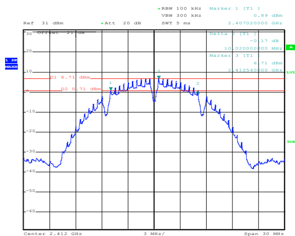
Figure 8.2-1: 6 dB bandwidth on 802.11b, sample plot – CCK: 1 Mbps
