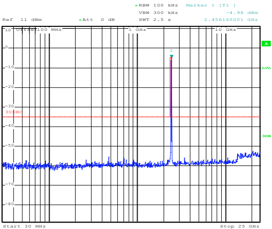
Figure 8.4-12: Conducted spurious emissions for 802.11n HT40 (TX 2452 MHz)
