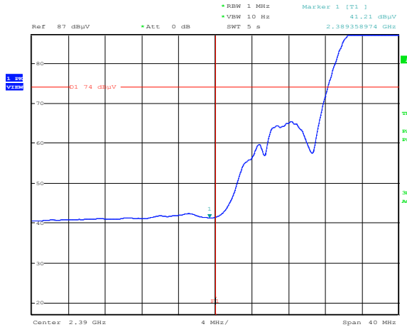
Figure 8.4-39: Radiated spurious emissions Lower band edge for 802.11b, (TX 2417 MHz) – Average
