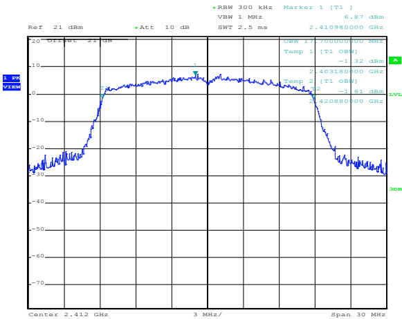
Figure 8.2-21: 99% bandwidth on 802.11n HT20, sample plot – OFDM: BPSK_1/2_6.5Mbps
