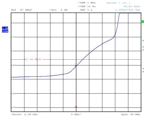
Figure 8.4-41: Radiated spurious emissions Lower band edge for 802.11g, (TX 2417 MHz) – Average
