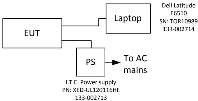
Figure 3.6-1: Setup diagram
