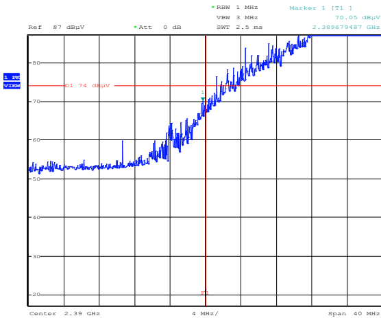
Figure 8.4-40: Radiated spurious emissions Lower band edge for 802.11g, (TX 2417 MHz) – Peak
