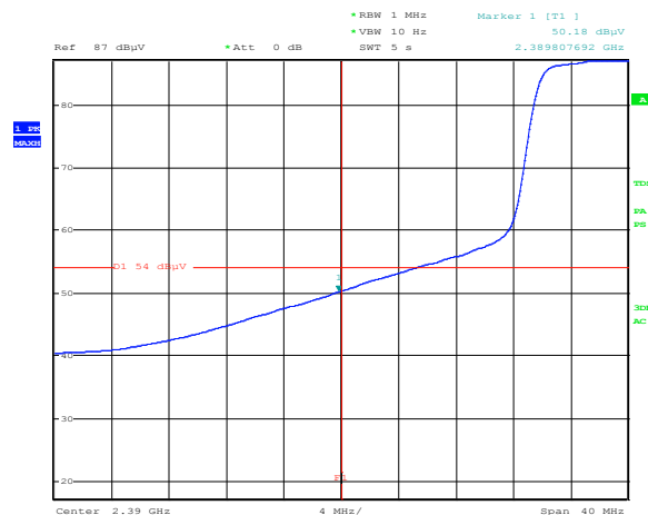
Figure 8.4-37: Radiated spurious emissions Lower band edge for 802.11n HT40, (TX 2422 MHz) – Average
