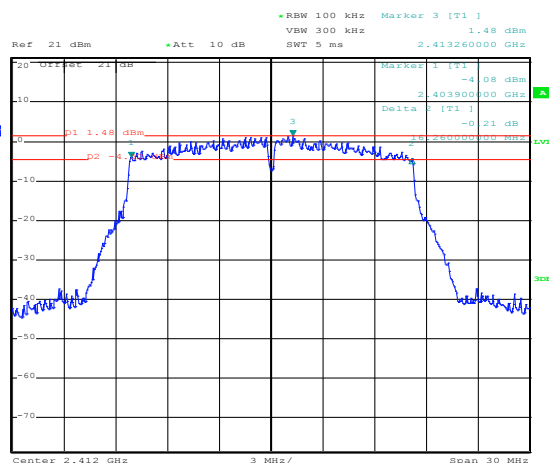
Figure 8.2-4: 6 dB bandwidth on 802.11g, sample plot – OFDM: QAM 64 3/4 54Mbps
