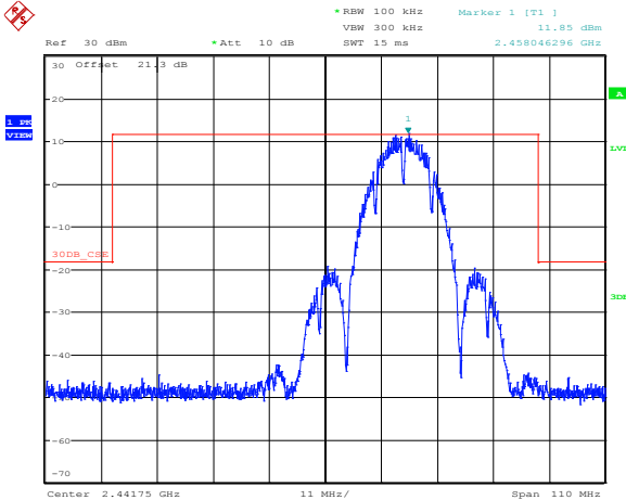
Figure 8.4-27: Conducted spurious emissions Upper band edge for 802.11b, (TX 2457 MHz)
