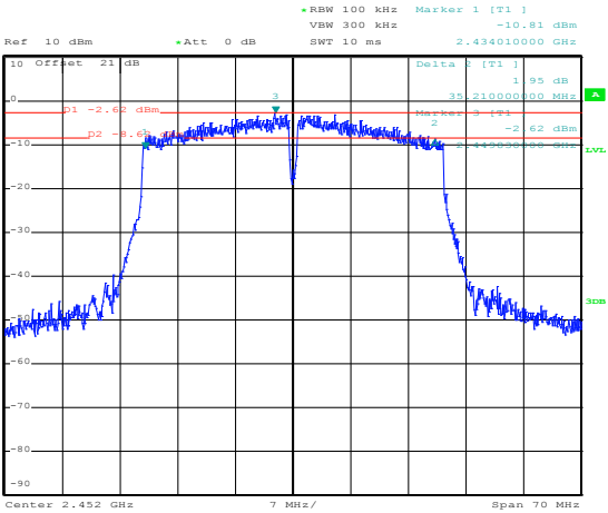
Figure 8.2-8: 6 dB bandwidth on 802.11n HT40, sample plot – OFDM: QAM 64_3/4_65Mbps
