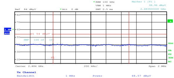
Figure 8.4-53: Radiated spurious emissions Upper band edge for 802.11b, (TX 2457 MHz) – Average
