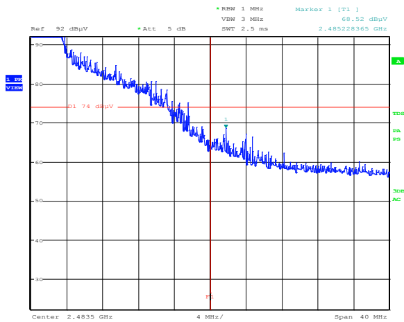
Figure 8.4-56: Radiated spurious emissions Upper band edge for 802.11n HT20, (TX 2457 MHz) – Peak
