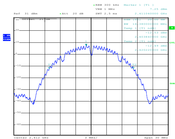
Figure 8.2-9: 20 dB bandwidth on 802.11b, sample plot – CCK: 1 Mbps
