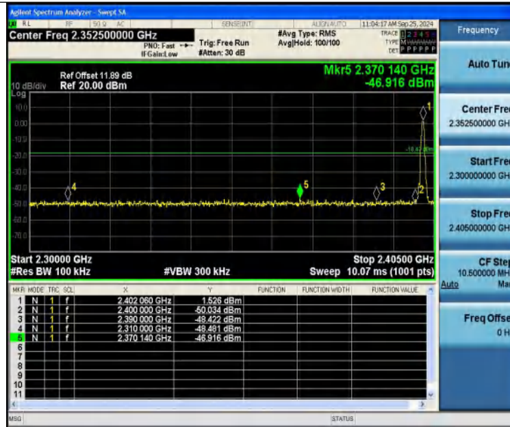
DH5-Ant1-2402-PASS
