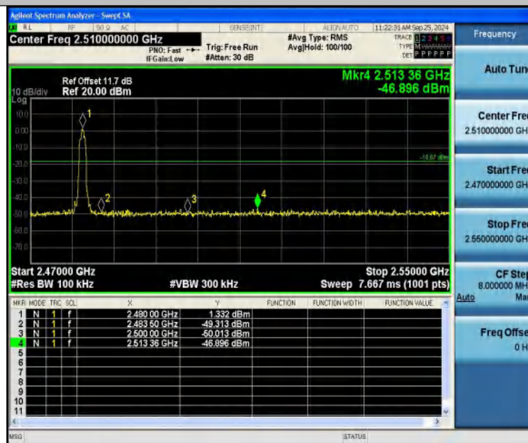
3DH5-Ant1-2480-PASS
