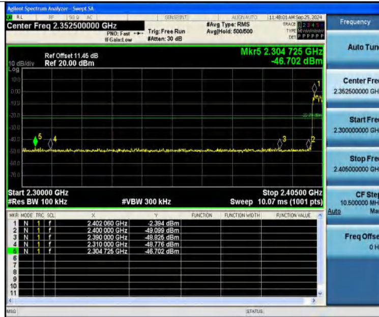
3DH5-Ant1-Hop_2402-PASS
