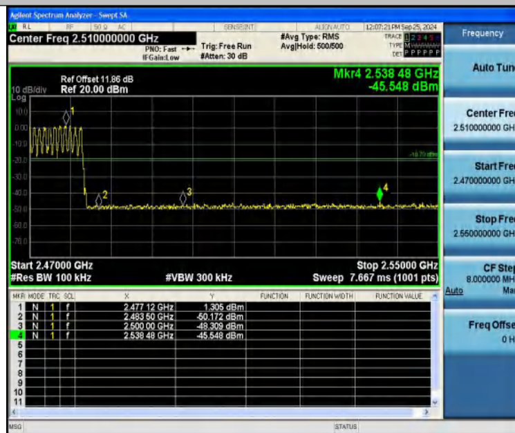
DH5-Ant1-Hop_2480-PASS
