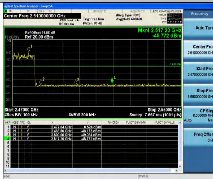
3DH5-Ant1-Hop_2480-PASS
