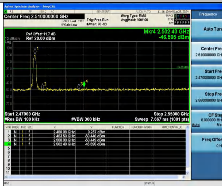
2DH5-Ant1-2480-PASS
