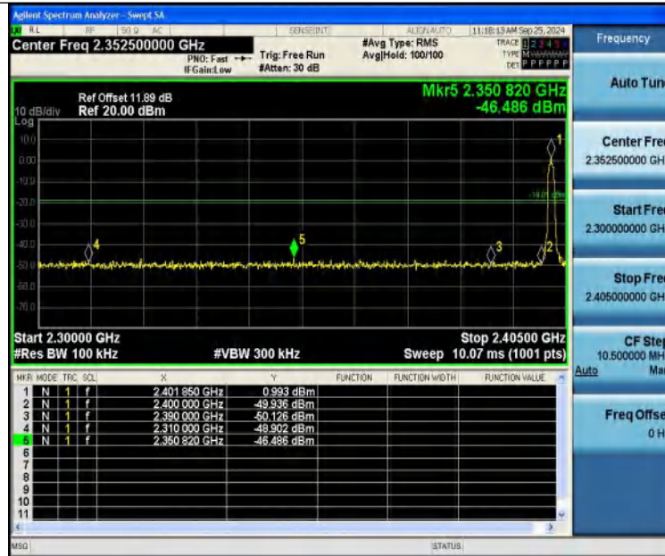
3DH5-Ant1-2402-PASS
