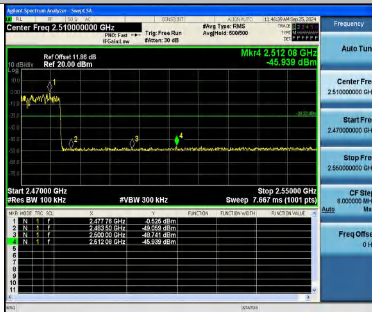
2DH5-Ant1-Hop_2480-PASS
