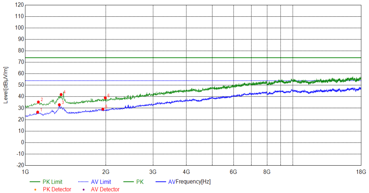
(Plot F: Test Antenna Vertical 1G – 18G)
