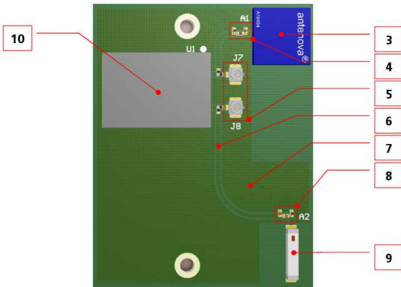
Figure 2: EMMY-W1 antenna reference design
