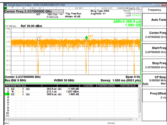
DUTY CYCLE 802.11g
