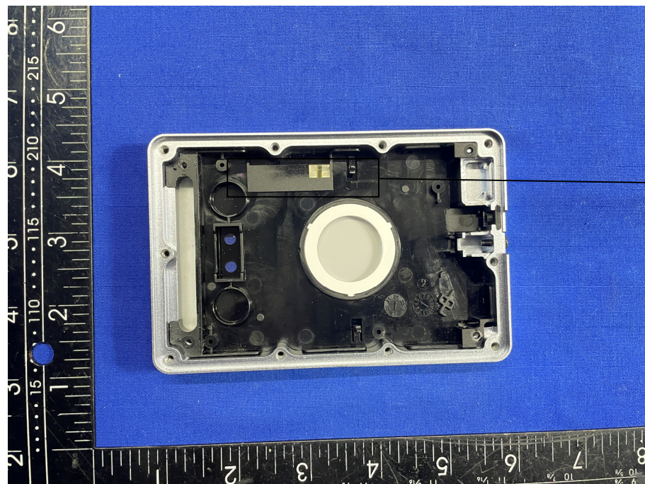
FPC Antenna Location
