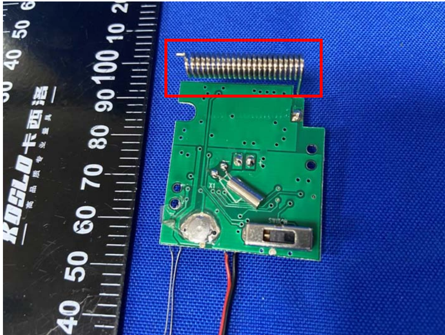
433.92 MHz TX Antenna
