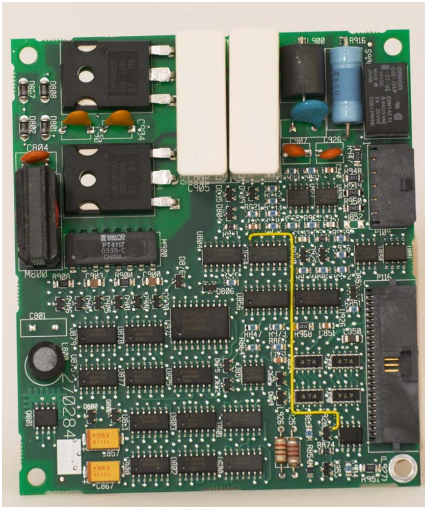
Inductive Telemetry Board Front
