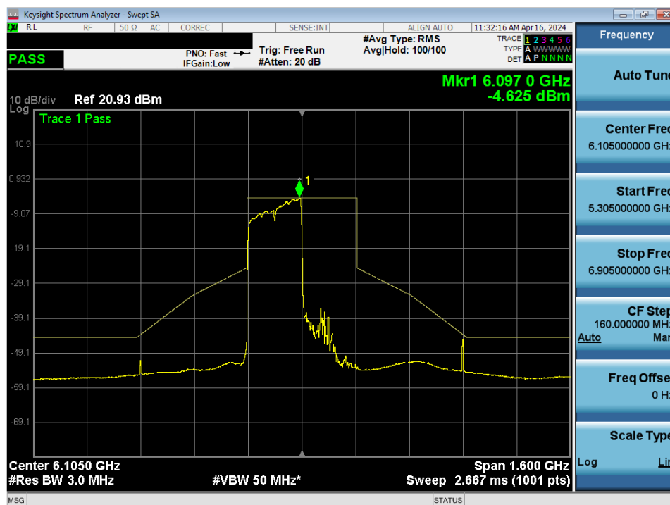
Plot 7-239. In-Band Emission Plot MIMO ANT1 (320MHz BW 802. 11be (Full Tones) (UNII Band 5) – Ch. 31) – LPI & SP
