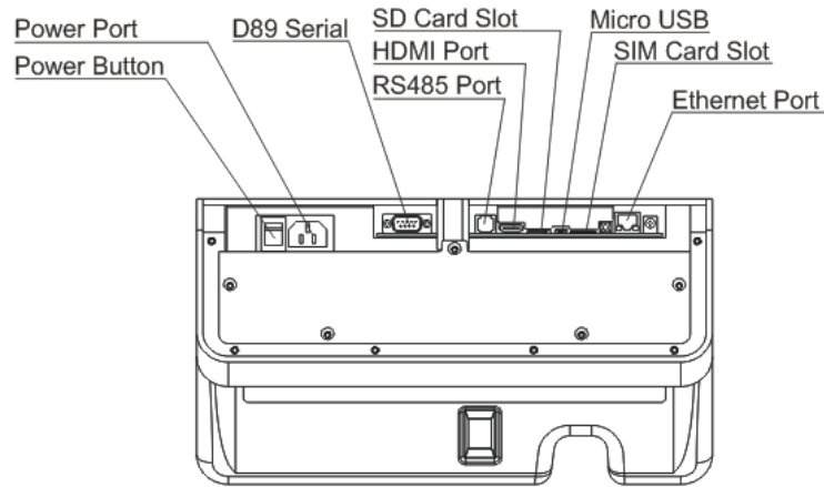
Interface Diagram
