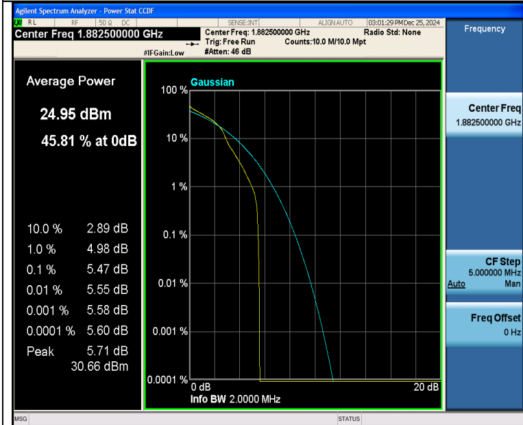
Band25-1.4MHz-16QAM-26365-1RB#0-PASS
