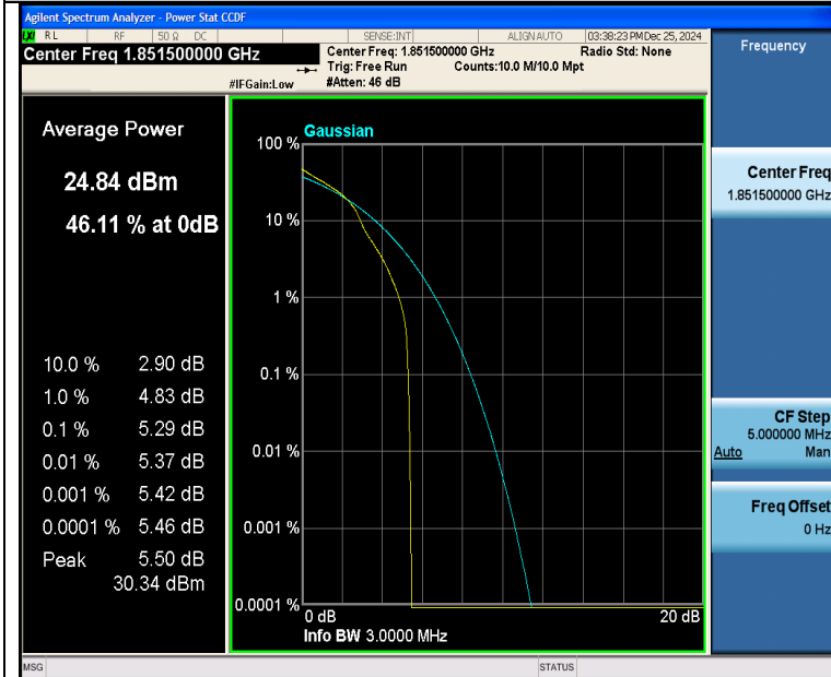
Band25-3MHz-16QAM-26055-1RB#0-PASS
