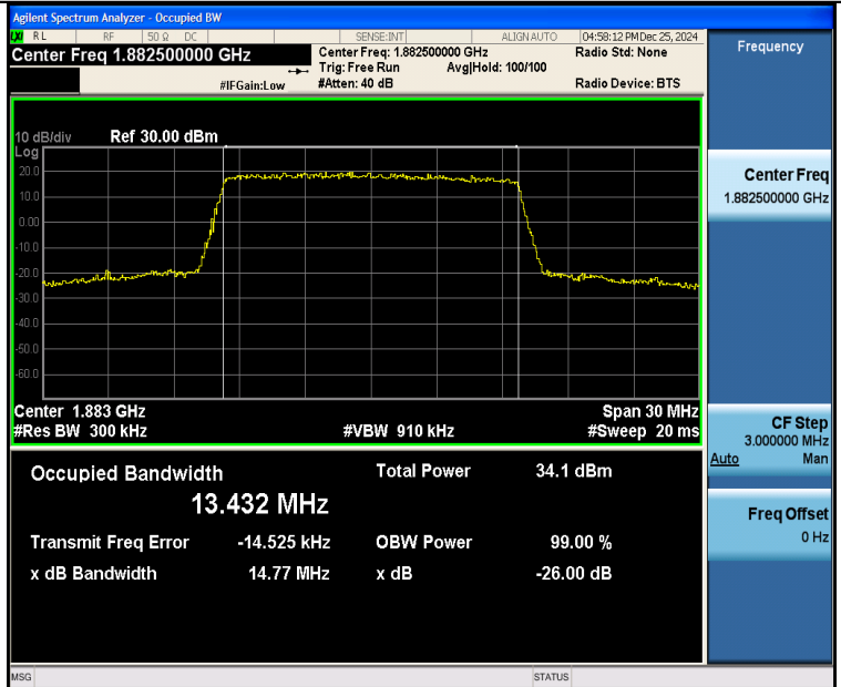
Band25-15MHz-QPSK-26365-75RB#0-PASS
