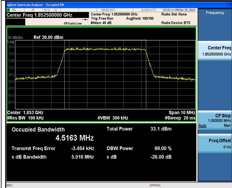
Band25-5MHz-QPSK-26065-25RB#0-PASS
