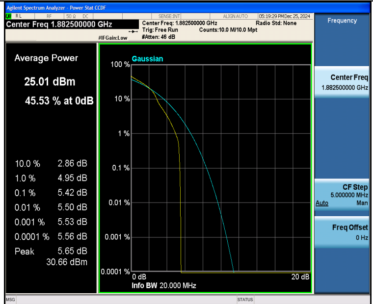
Band25-15MHz-16QAM-26365-1RB#0-PASS
