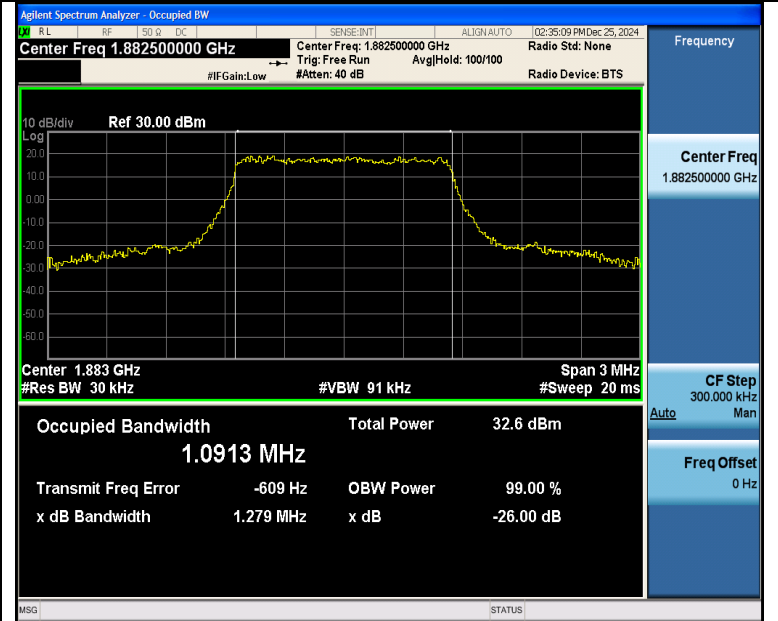
Band25-1.4MHz-16QAM-26365-6RB#0-PASS
