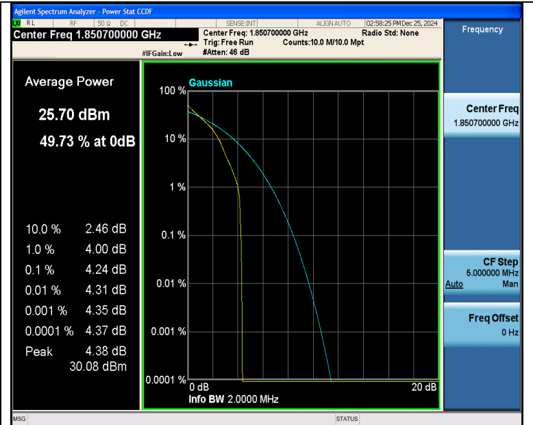
Band25-1.4MHz-QPSK-26047-1RB#0-PASS
