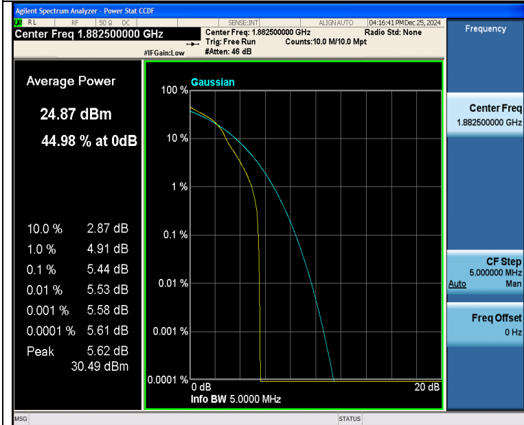
Band25-5MHz-16QAM-26365-1RB#0-PASS
