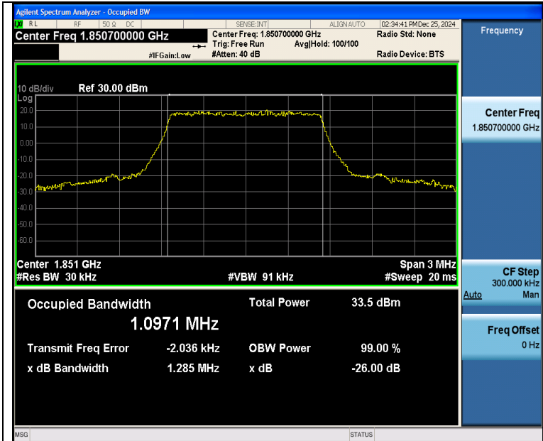
Band25-1.4MHz-QPSK-26047-6RB#0-PASS
