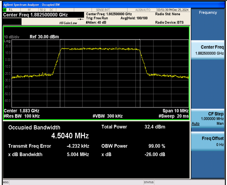
Band25-5MHz-16QAM-26365-25RB#0-PASS
