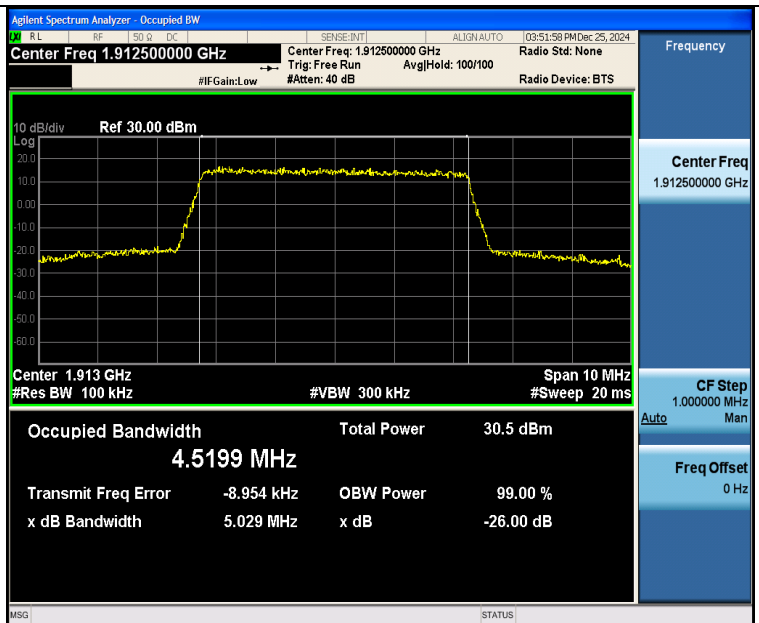
Band25-5MHz-16QAM-26665-25RB#0-PASS
