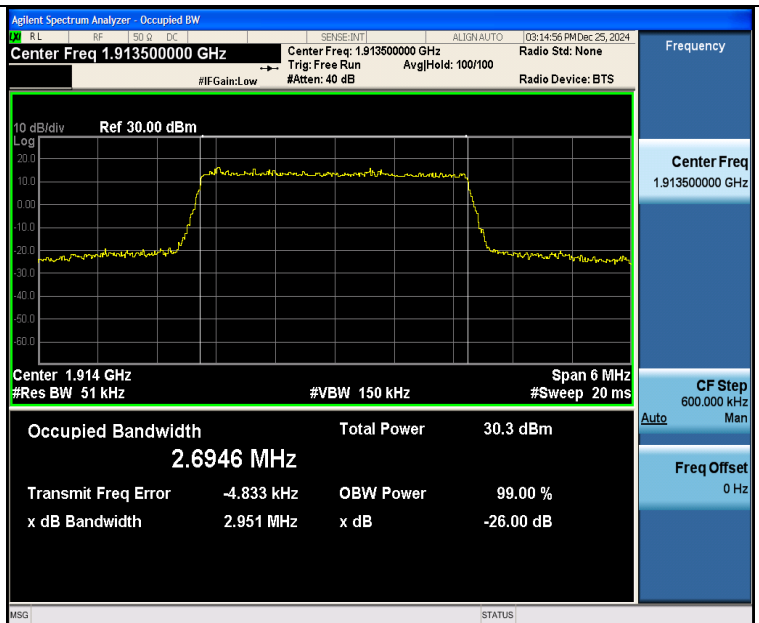
Band25-3MHz-16QAM-26675-15RB#0-PASS
