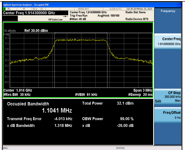
Band25-1.4MHz-16QAM-26683-6RB#0-PASS
