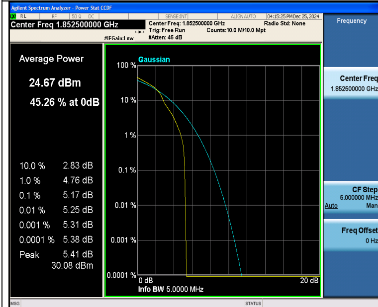
Band25-5MHz-16QAM-26065-1RB#0-PASS
