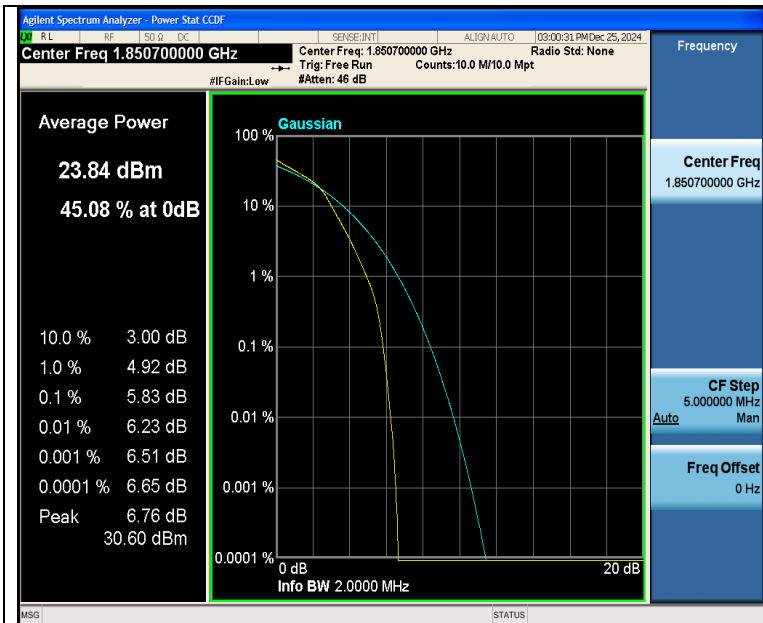
Band25-1.4MHz-16QAM-26047-6RB#0-PASS
