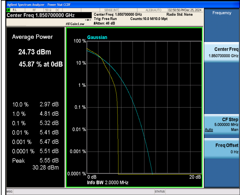
Band25-1.4MHz-16QAM-26047-1RB#0-PASS
