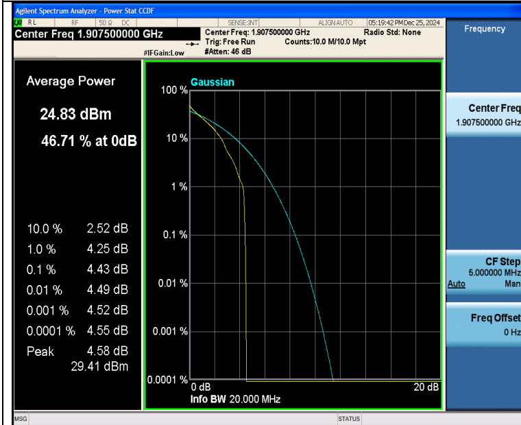
Band25-15MHz-QPSK-26615-1RB#0-PASS
