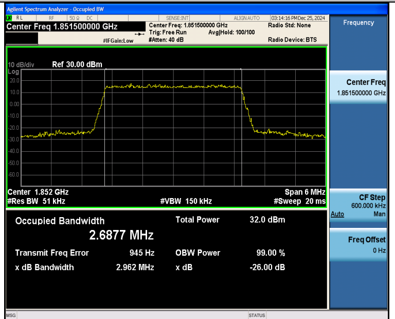
Band25-3MHz-16QAM-26055-15RB#0-PASS
