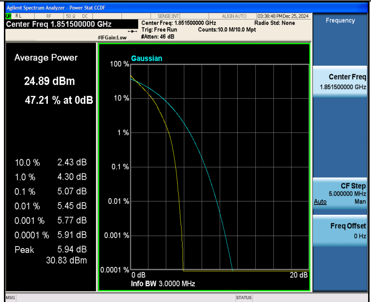
Band25-3MHz-QPSK-26055-15RB#0-PASS
