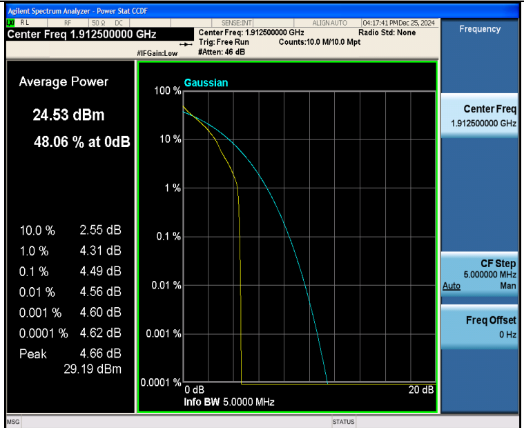
Band25-5MHz-QPSK-26665-1RB#0-PASS
