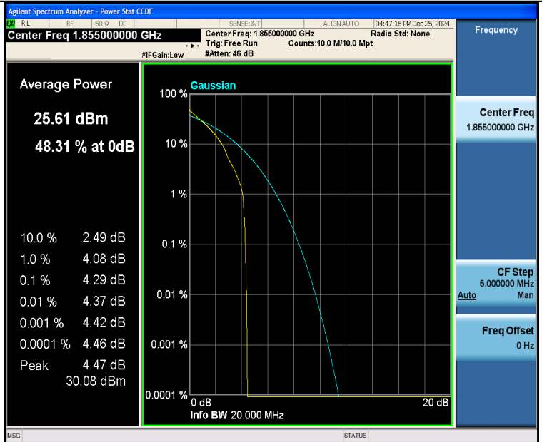
Band25-10MHz-QPSK-26090-1RB#0-PASS
