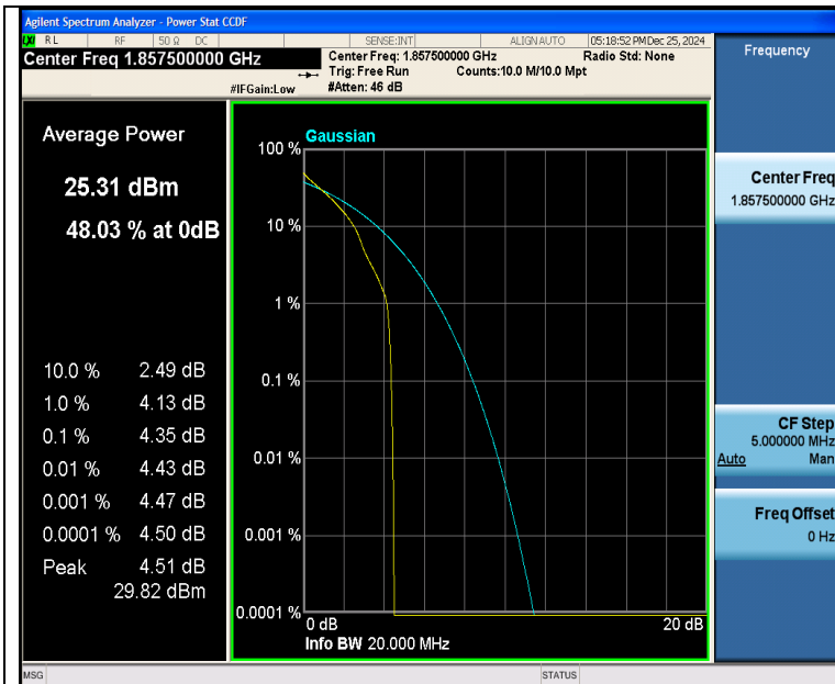
Band25-15MHz-QPSK-26115-1RB#0-PASS
