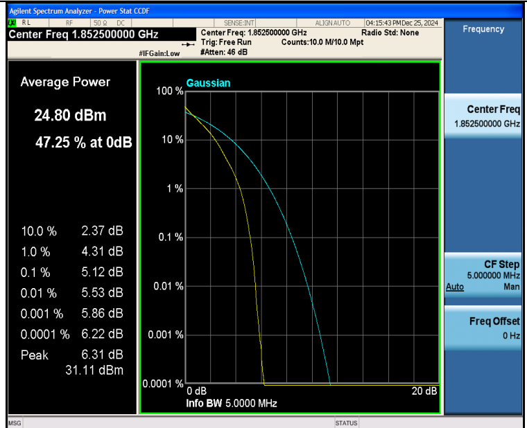
Band25-5MHz-QPSK-26065-25RB#0-PASS
