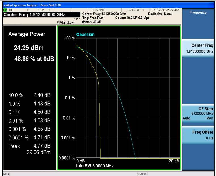
Band25-3MHz-QPSK-26675-1RB#0-PASS
