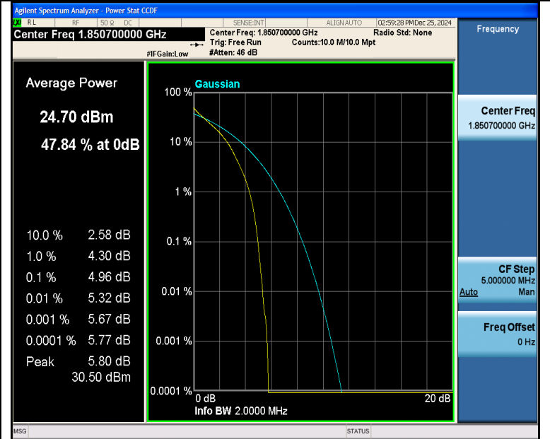
Band25-1.4MHz-QPSK-26047-6RB#0-PASS
