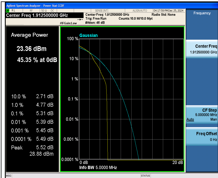
Band25-5MHz-16QAM-26665-1RB#0-PASS
