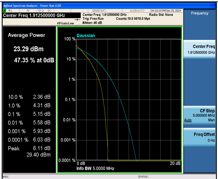
Band25-5MHz-QPSK-26665-25RB#0-PASS
