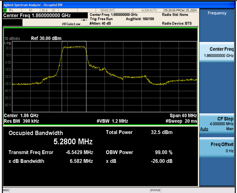
Band25-20MHz-16QAM-26140-27RB#0-PASS
