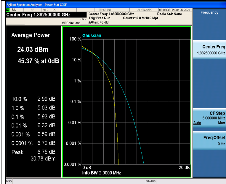
Band25-1.4MHz-16QAM-26365-6RB#0-PASS
