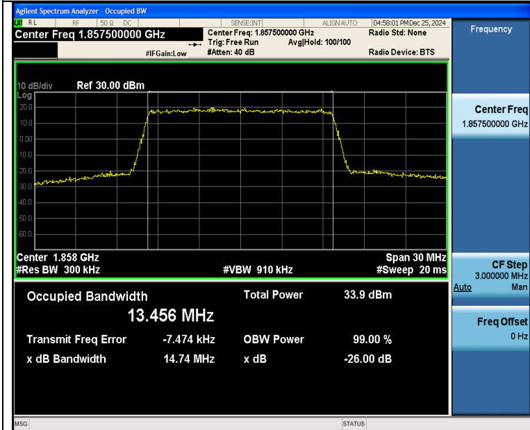
Band25-15MHz-QPSK-26115-75RB#0-PASS
