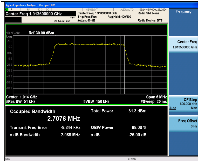
Band25-3MHz-QPSK-26675-15RB#0-PASS
