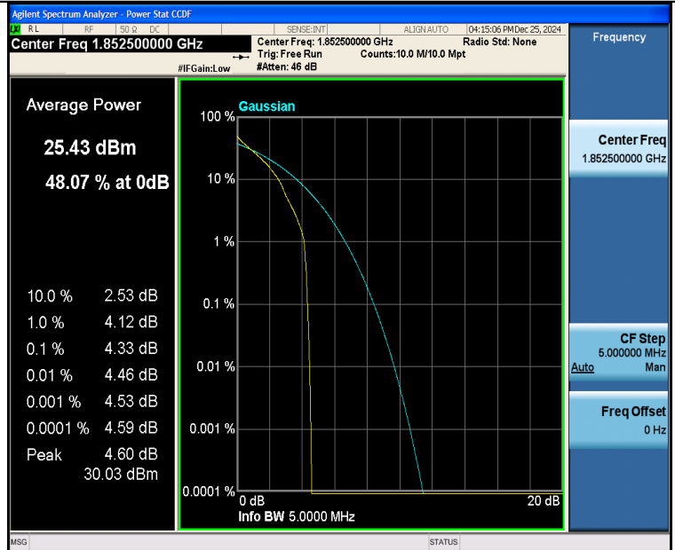
Band25-5MHz-QPSK-26065-1RB#0-PASS
