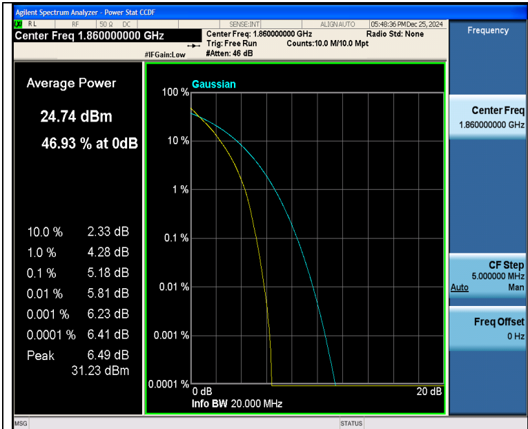
Band25-20MHz-QPSK-26140-100RB#0-PASS
