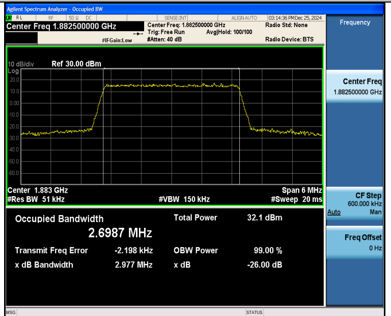
Band25-3MHz-16QAM-26365-15RB#0-PASS
