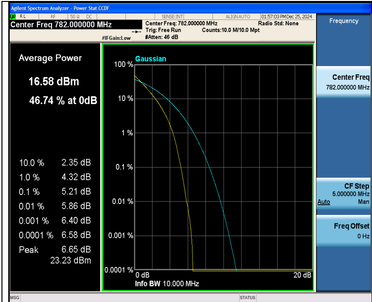
Band13-10MHz-QPSK-23230-50RB#0-PASS
