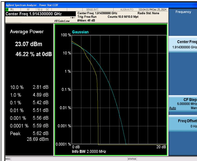
Band25-1.4MHz-16QAM-26683-1RB#0-PASS
