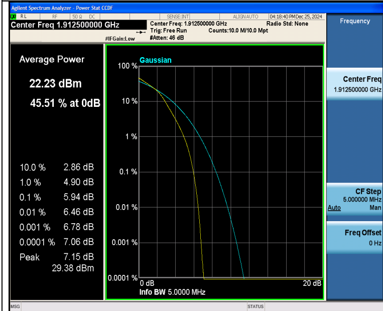
Band25-5MHz-16QAM-26665-25RB#0-PASS
