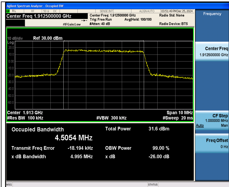
Band25-5MHz-QPSK-26665-25RB#0-PASS
