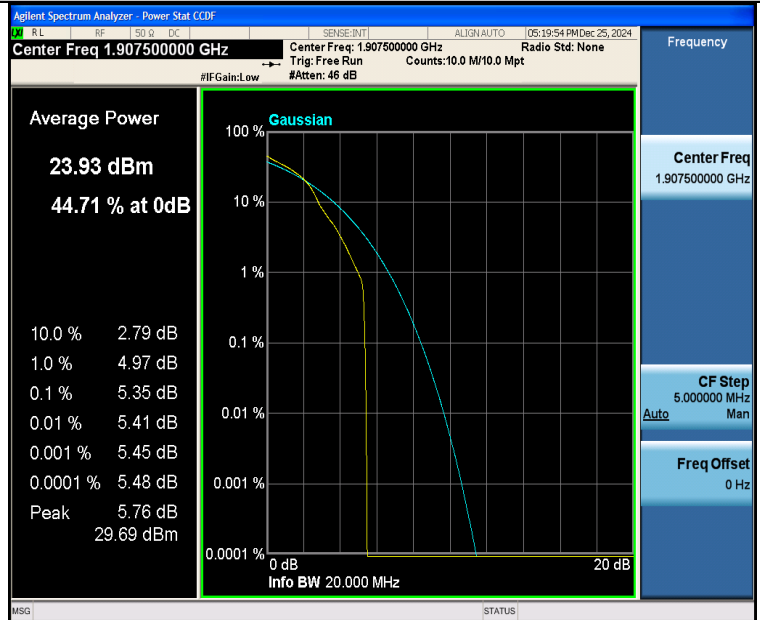
Band25-15MHz-16QAM-26615-1RB#0-PASS
