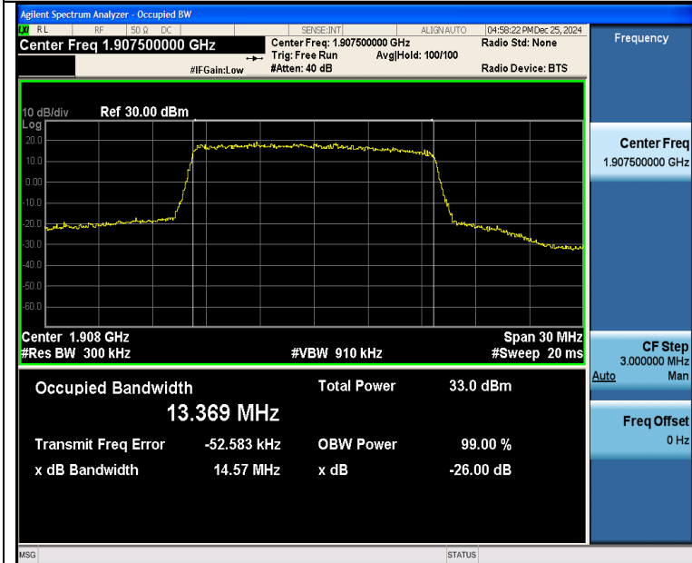
Band25-15MHz-QPSK-26615-75RB#0-PASS
