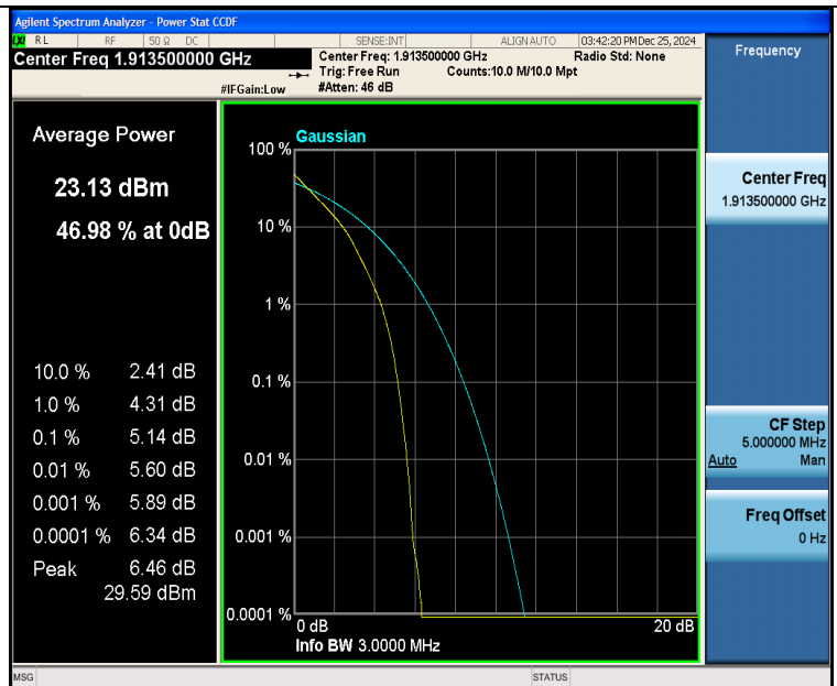
Band25-3MHz-QPSK-26675-15RB#0-PASS
