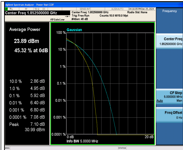
Band25-5MHz-16QAM-26065-25RB#0-PASS
