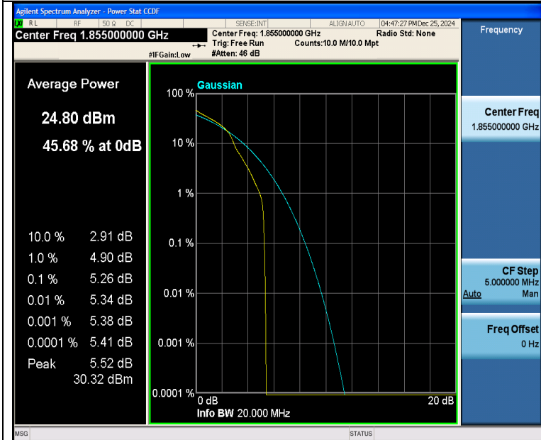
Band25-10MHz-16QAM-26090-1RB#0-PASS
