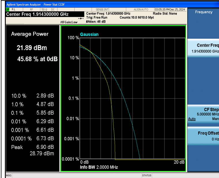
Band25-1.4MHz-16QAM-26683-6RB#0-PASS
