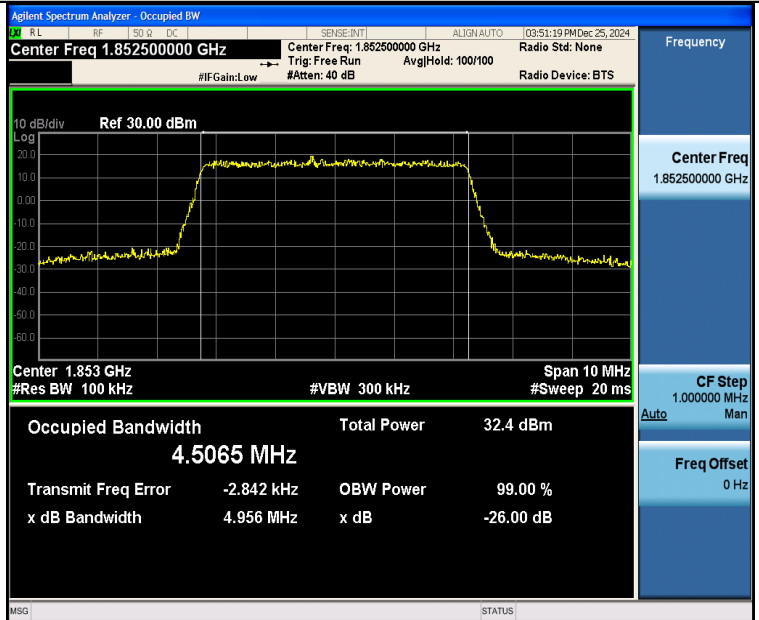
Band25-5MHz-16QAM-26065-25RB#0-PASS
