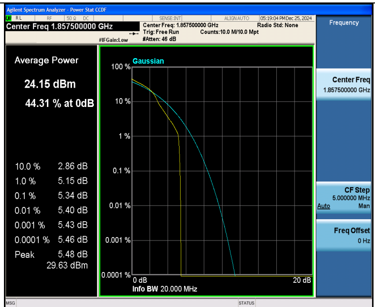
Band25-15MHz-16QAM-26115-1RB#0-PASS
