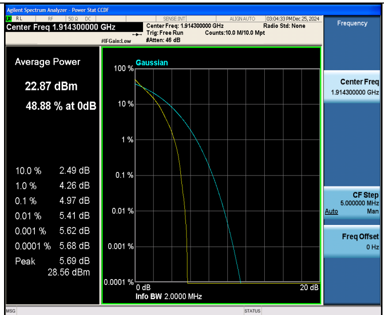
Band25-1.4MHz-QPSK-26683-6RB#0-PASS
