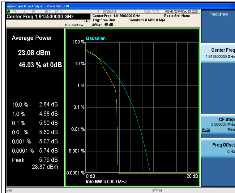
Band25-3MHz-16QAM-26675-1RB#0-PASS
