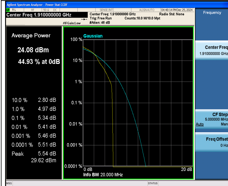
Band25-10MHz-16QAM-26640-1RB#0-PASS
