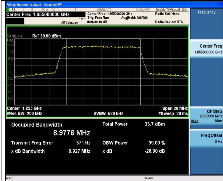
Band25-10MHz-QPSK-26090-50RB#0-PASS
