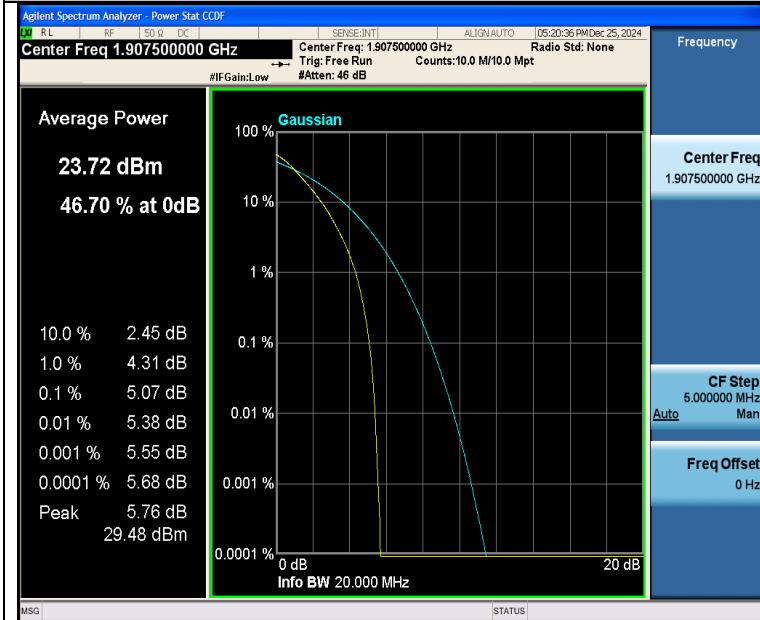
Band25-15MHz-QPSK-26615-75RB#0-PASS
