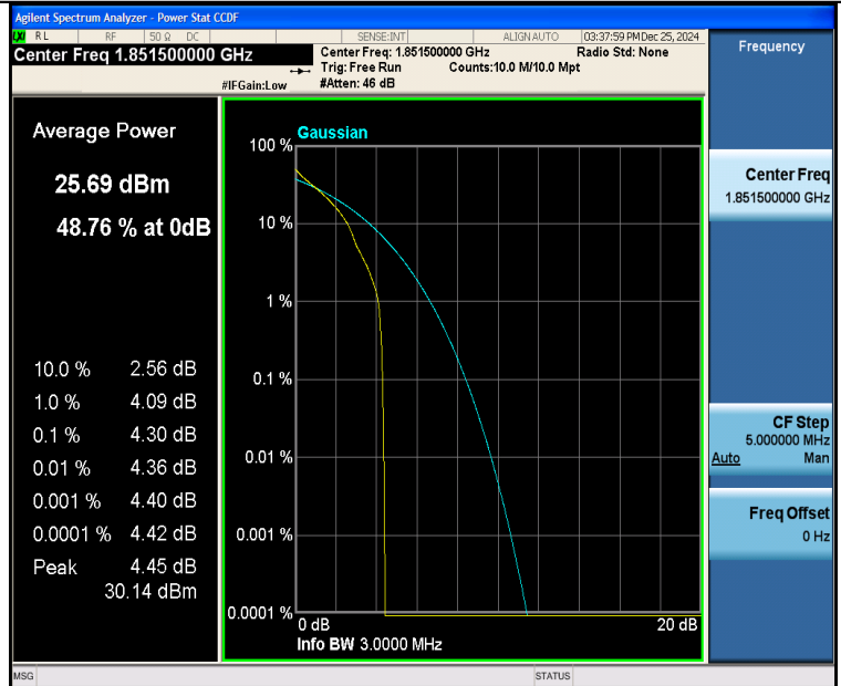
Band25-3MHz-QPSK-26055-1RB#0-PASS
