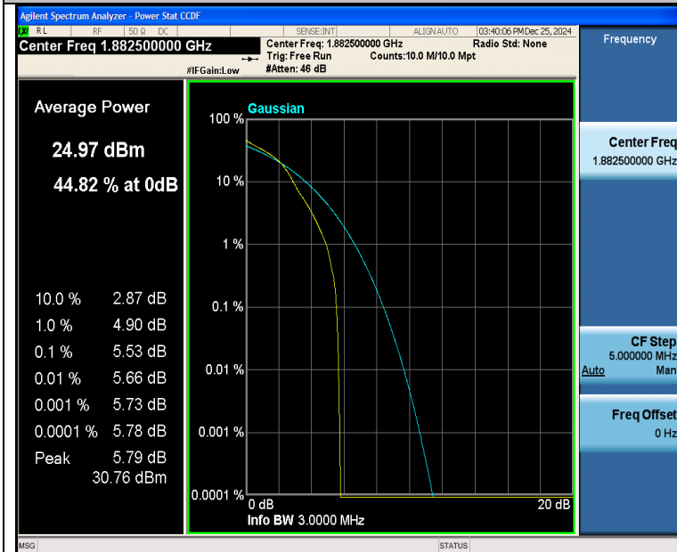
Band25-3MHz-16QAM-26365-1RB#0-PASS
