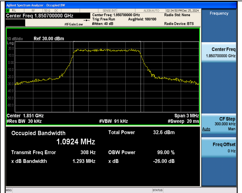
Band25-1.4MHz-16QAM-26047-6RB#0-PASS
