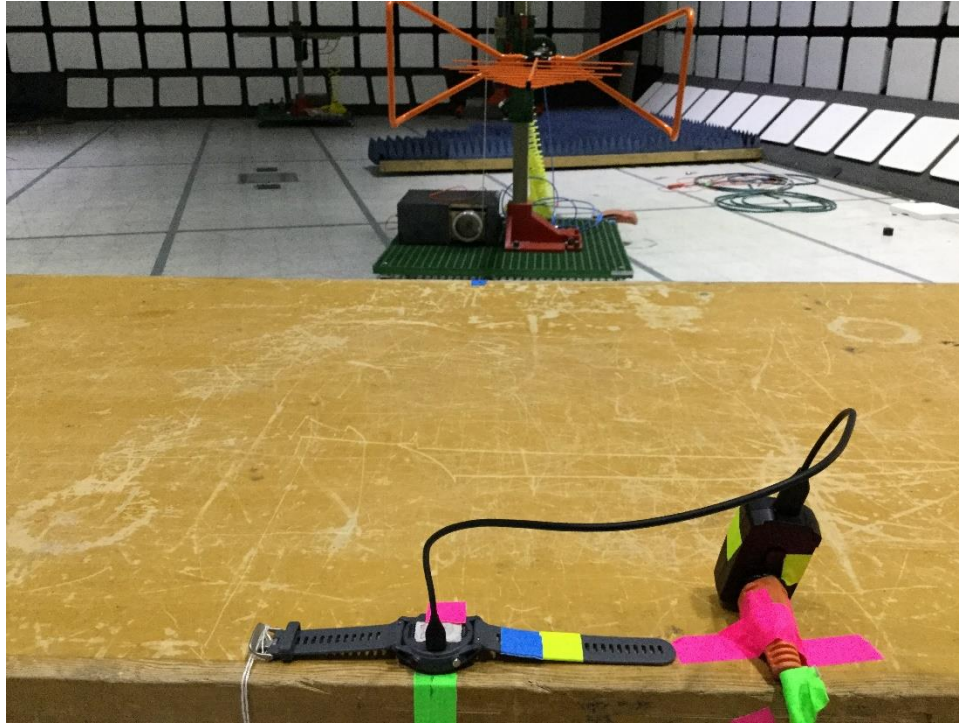
30 MHz – 1 GHz Test Setup
