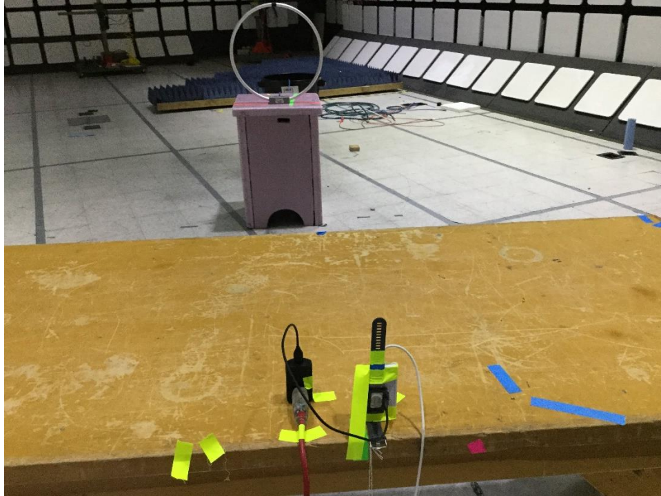
150kHz – 30 MHz Test Setup
