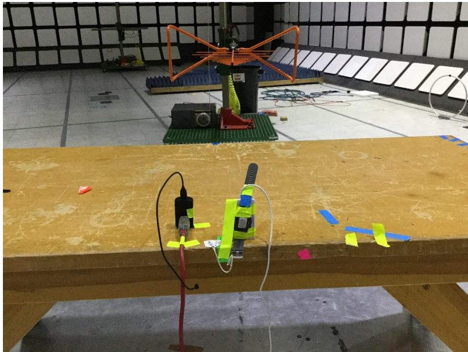
30 MHz – 1 GHz Test Setup, NFC
