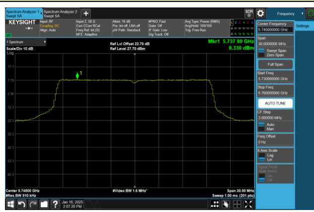
Channel 149 (5745MHz)
