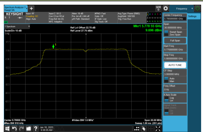
Channel 157 (5785MHz)
