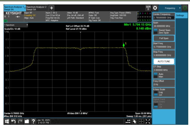
Channel 157 (5785MHz)
