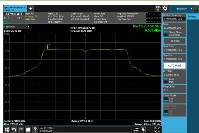
Channel 149 (5745MHz)
