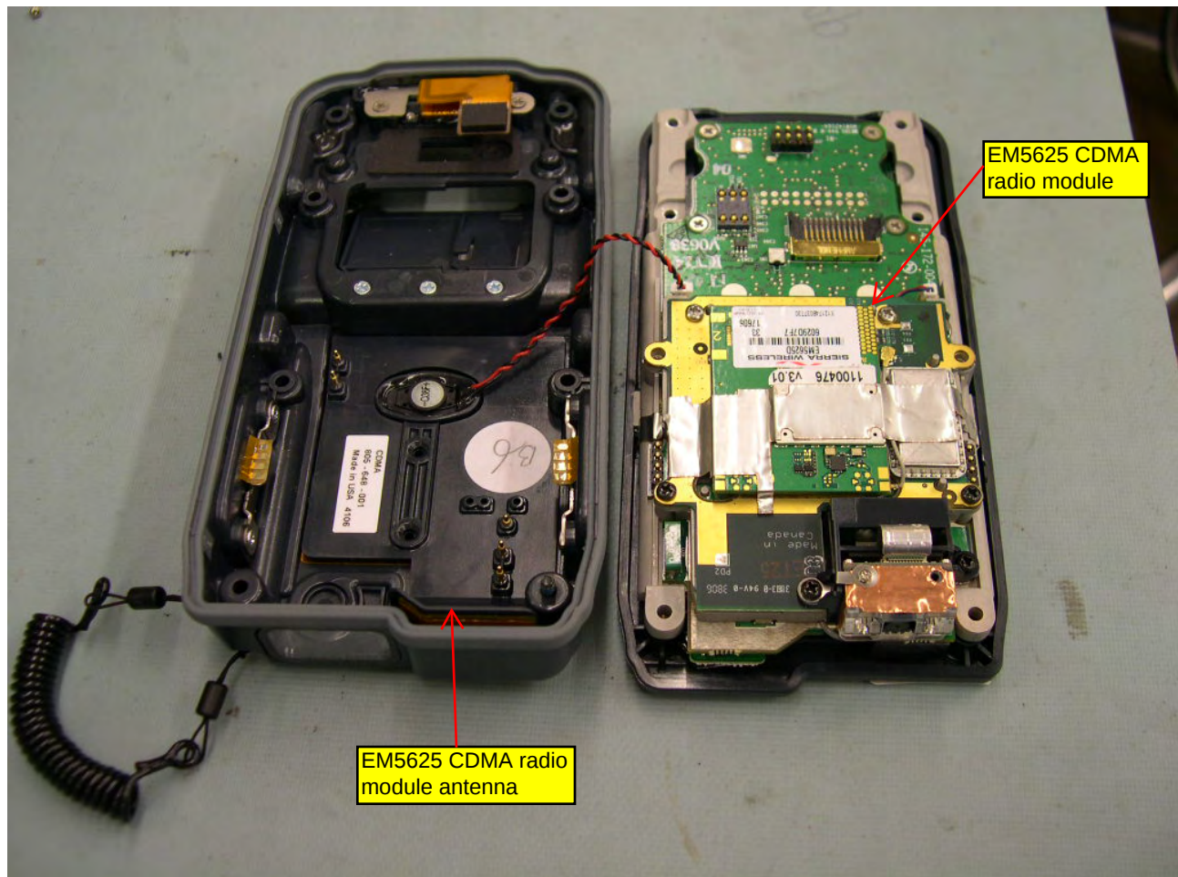
CN3 Case Open showing EM5625 and Antenna
