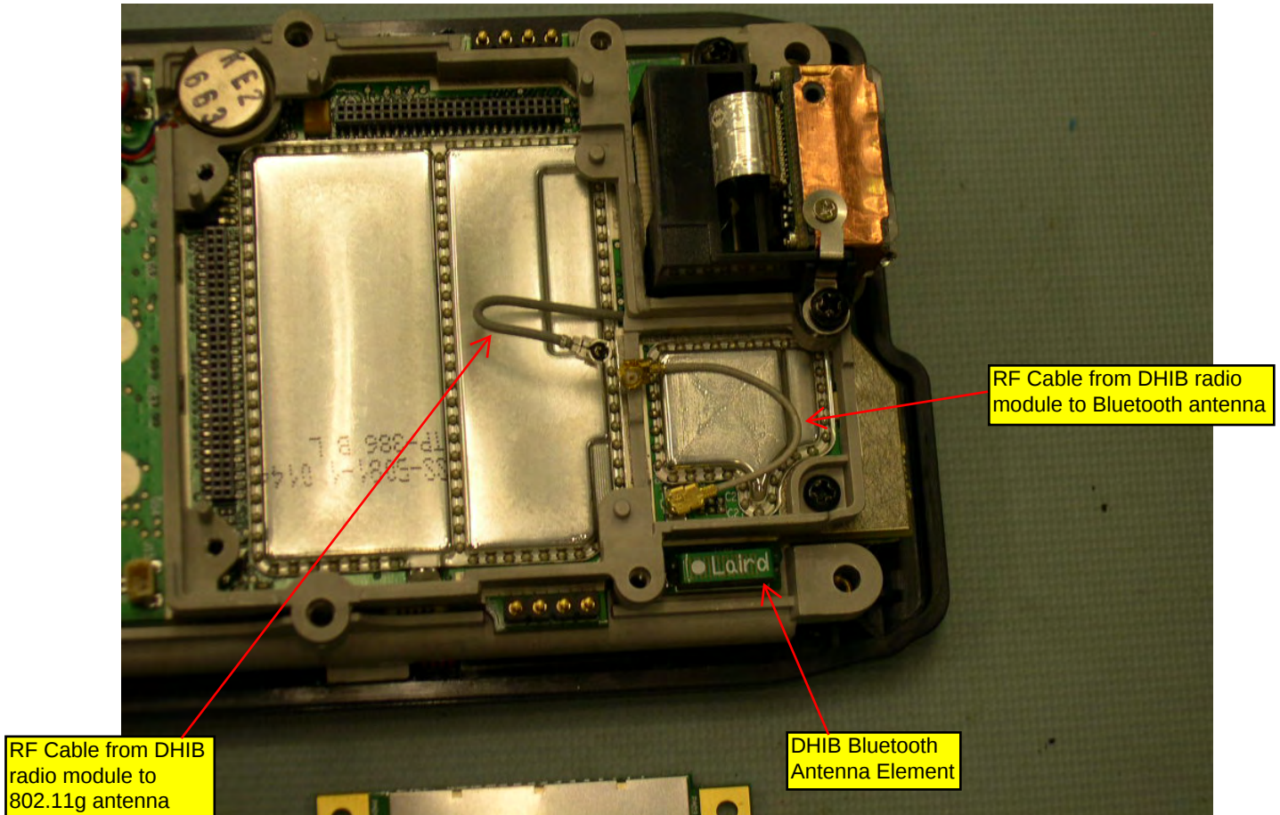
\ CN3 Unit with MC75 and DHIB modules removed to show DHIB RF cables
