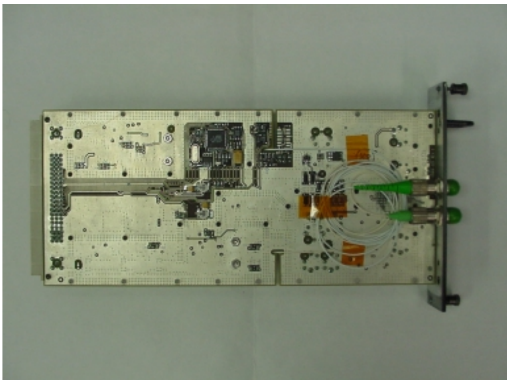
Fibre Optic Control Module Bottom
