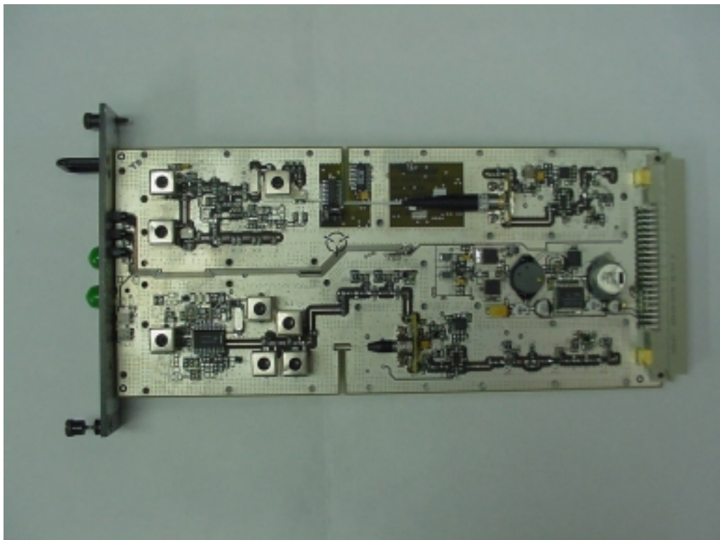
Fibre Optic Control Module Top
