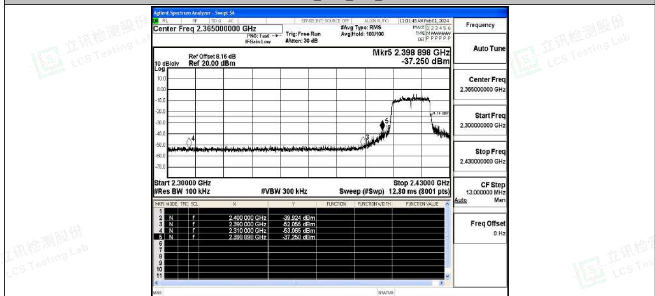
11N20SISO_Ant0_Low_2412
