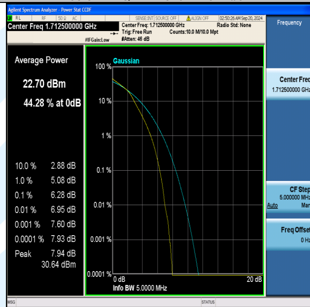
Band66-5MHz-16QAM-131997-25RB#0-PASS
