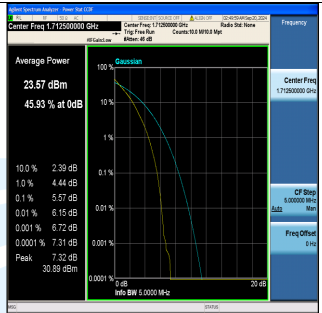
Band66-5MHz-QPSK-131997-25RB#0-PASS
