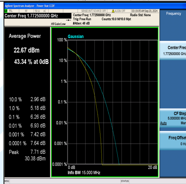
Band66-15MHz-16QAM-132597-75RB#0-PASS
