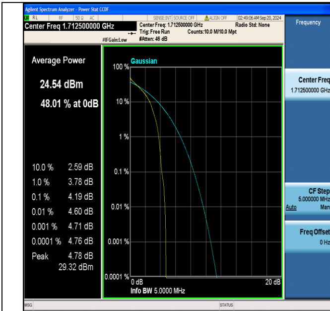
Band66-5MHz-QPSK-131997-1RB#0-PASS
