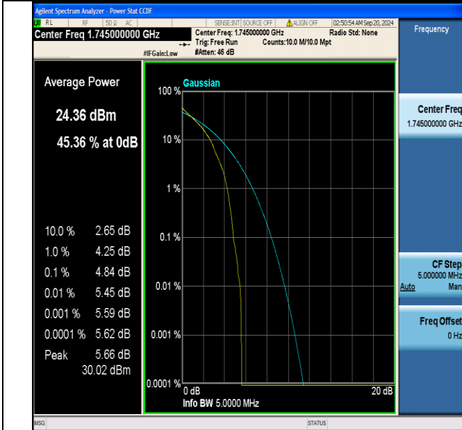
Band66-5MHz-QPSK-132322-1RB#0-PASS
