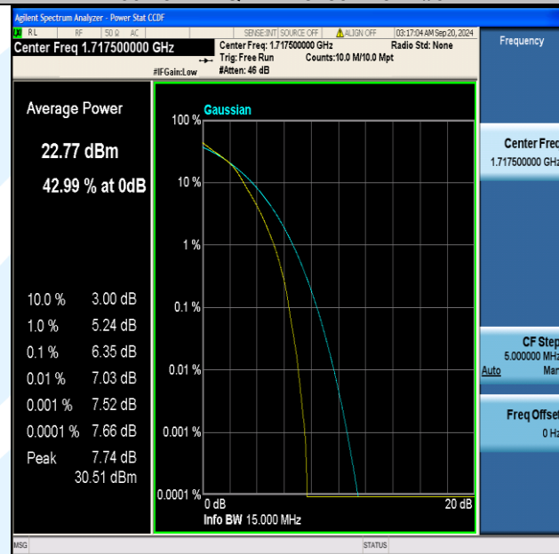
Band66-15MHz-16QAM-132047-75RB#0-PASS
