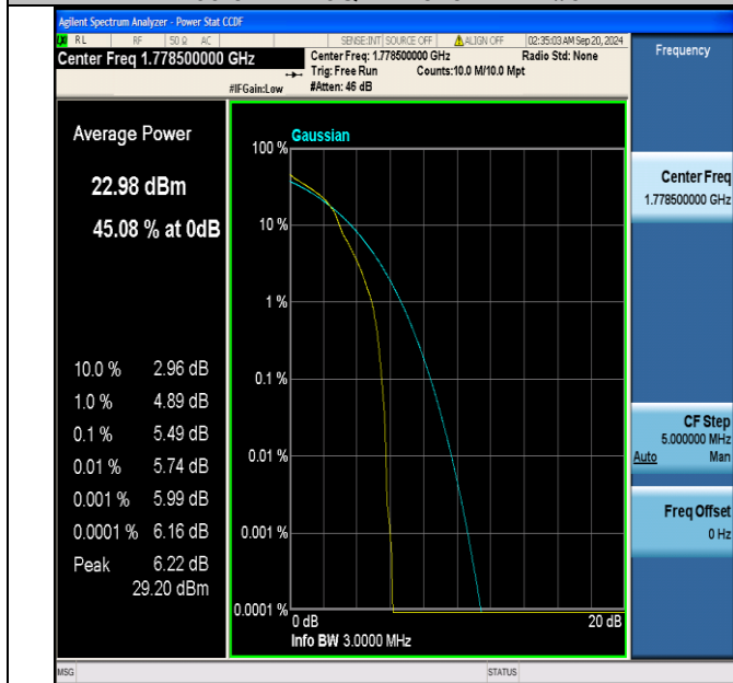
Band66-3MHz-16QAM-132657-1RB#0-PASS
