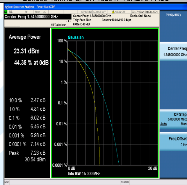
Band66-15MHz-QPSK-132322-75RB#0-PASS
