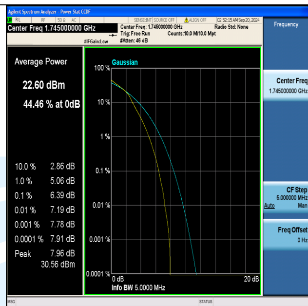
Band66-5MHz-16QAM-132322-25RB#0-PASS
