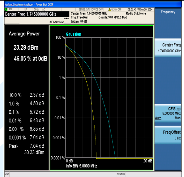
Band66-5MHz-QPSK-132322-25RB#0-PASS
