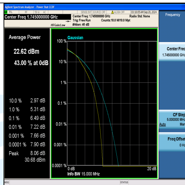
Band66-15MHz-16QAM-132322-75RB#0-PASS
