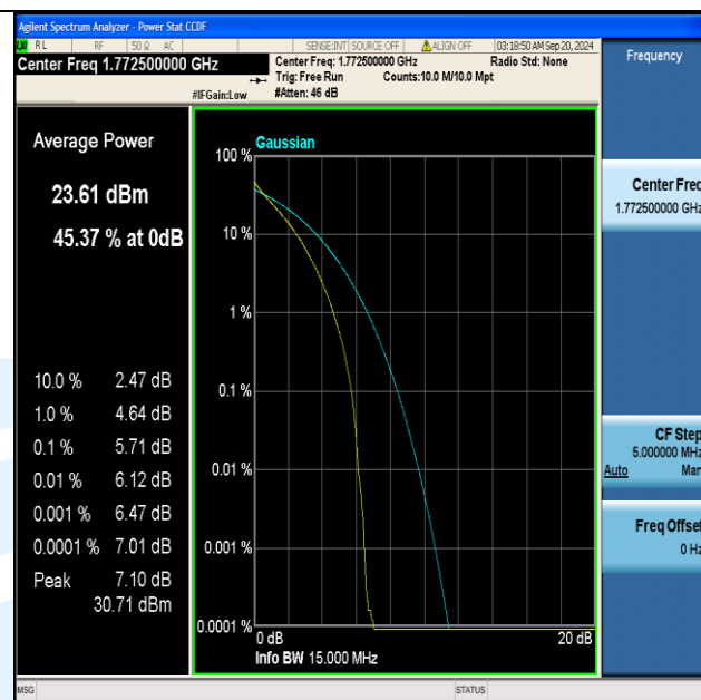
Band66-15MHz-QPSK-132597-75RB#0-PASS
