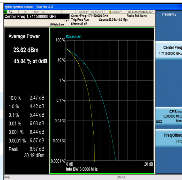
Band66-3MHz-QPSK-131987-15RB#0-PASS
