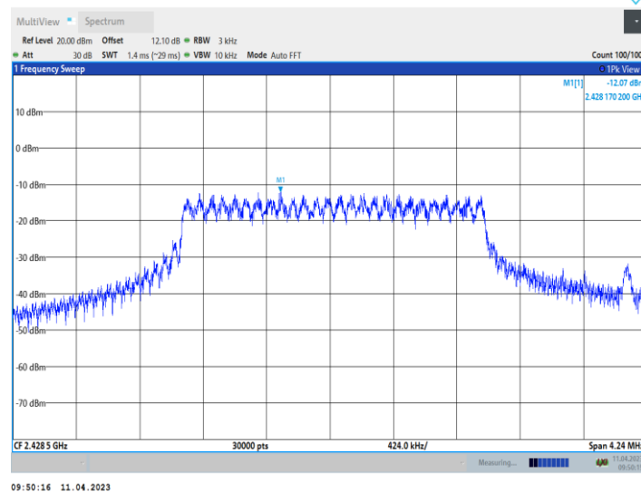
11AX20_Ant10_2437_52Tone_RU37
