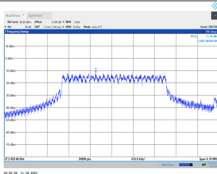
11AX20_Ant10_2462_52Tone_RU37
