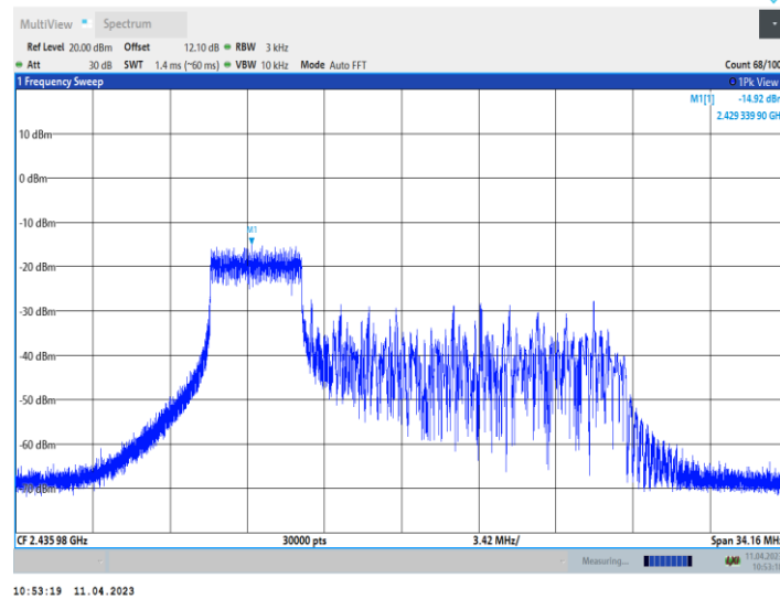
11AX20_Ant10_2437_106Tone_RU53
