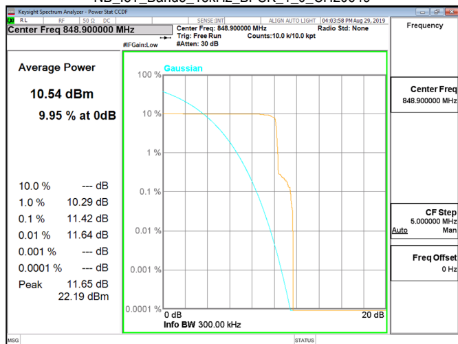
NB_IoT_Band5_15kHz_BPSK_1_0_CH20649
