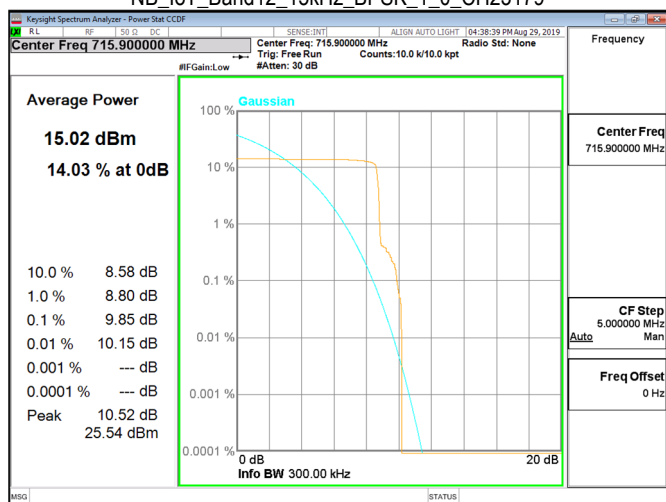
NB IoT_Band12_15kHz_BPSK_1_0_CH23179
