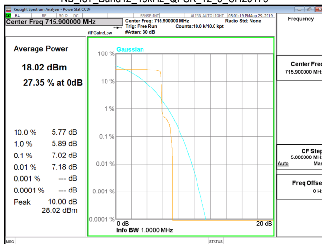
NB IoT_Band12_15kHz_QPSK_12_0_CH23179
