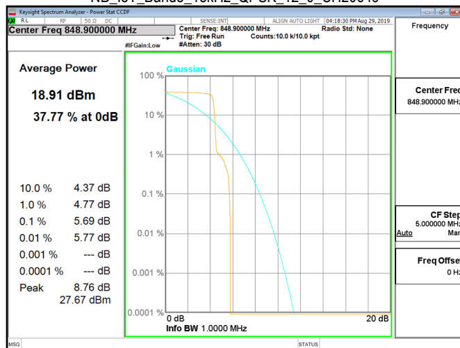
NB_IoT_Band5_15kHz_QPSK_12_0_CH20649
