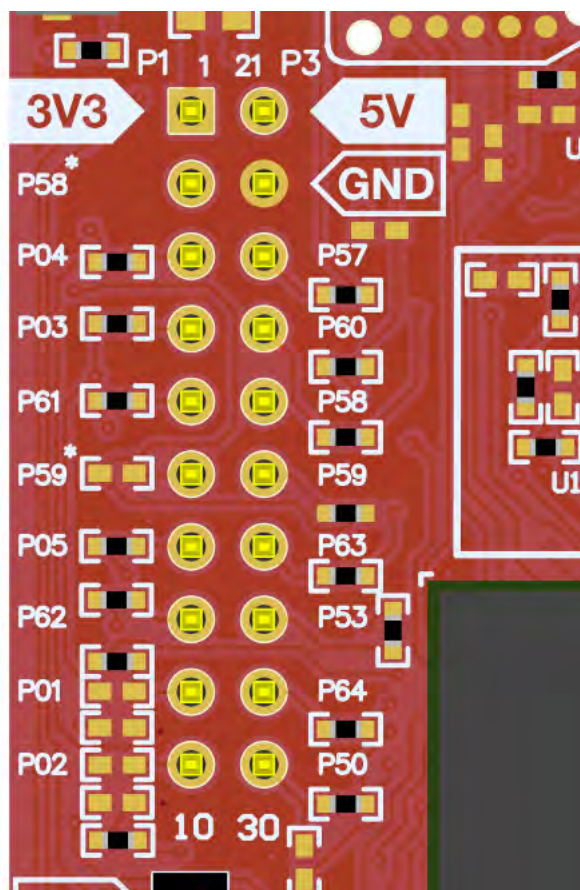
Figure 25. Pin 1 Marking on LaunchPad (3V3 Mark)
