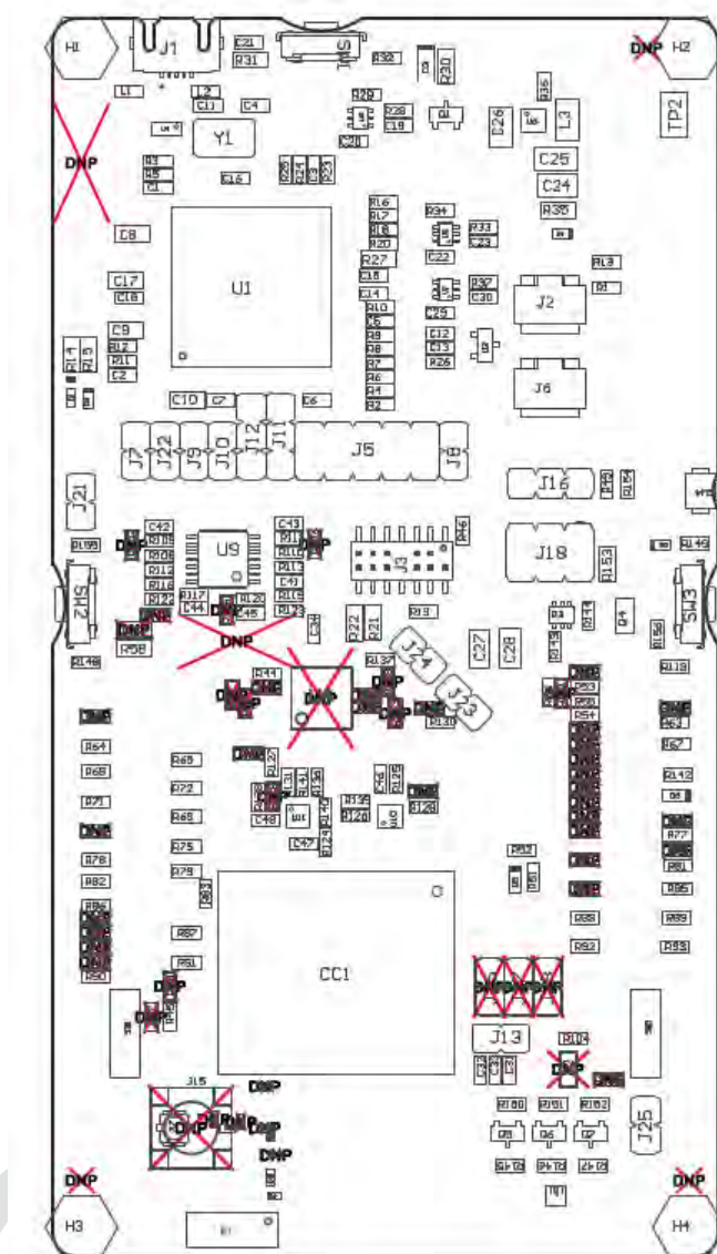
Figure 31. LAUNCHCC3235MOD Top-Layer Assembly Drawing
