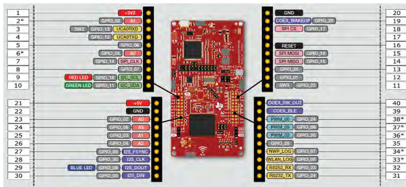
Figure 16. LAUNCHCC3235MOD BoosterPack™ Header Pin Assignments
