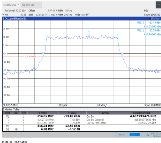
1-N26-814-824--15-5-L-3-DFT-16QAM-Outet_Full-25 @0-Ant1-4.468-4.980-≤5-PASS
