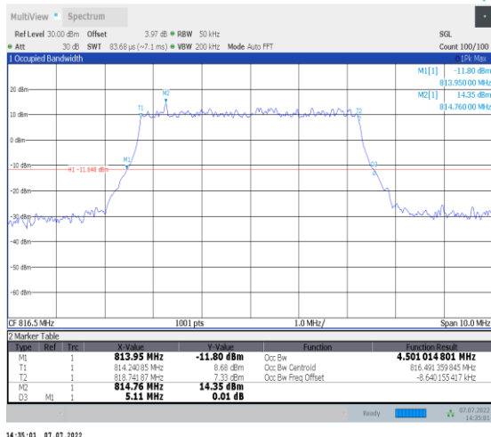
1-N26-814-824--15-5-L-1-DFT-QPSK-Outet_Full-25 @0-Ant1-4.501-5.110-≤5-PASS
