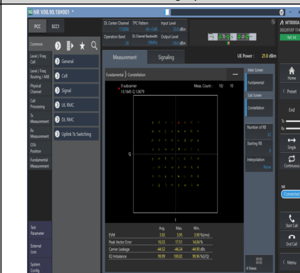
1-N26-814-824--15-10-M-8-CP-64QAM-Outer_Full-52@0-Ant1-see graph-PASS
