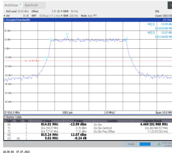
1-N26-814-824--15-5-L-4-DFT-64QAM-Outet_Full-2 5@0-Ant1-4.469-5.020-≤5-PASS
