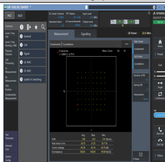
1-N26-814-824--15-10-M-4-DFT-64QAM-Out-50@0-Ant1-see graph-PASS
