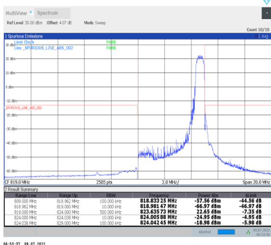
1-N26-814-824--15-5-H-5-CP-QPSK-Edge_1RB_Right-1@24-Ant1-PASS-see graph
