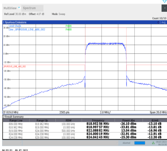
1-N26-814-824--15-5-H-6-CP-QPSK-Outer_Full-25@0-Ant1-PASS-see graph
