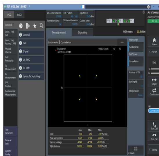
1-N26-814-824--15-10-M-2-DFT-QPSK-Out-0@0-Ant1-see graph-PASS
