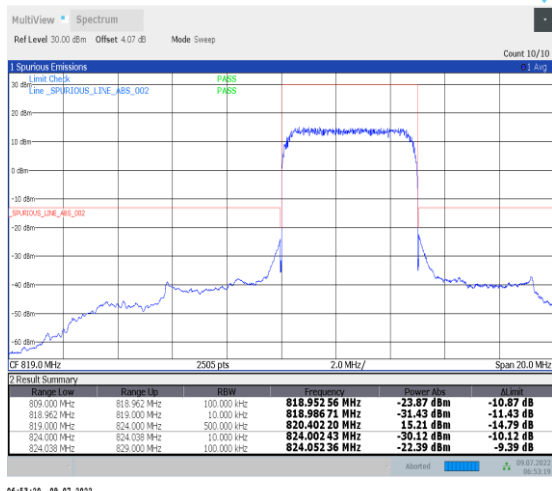
1-N26-814-824--15-5-H-3-DFT-PI2BPSK-Outer_Full-25@0-Ant1-PASS-see graph
