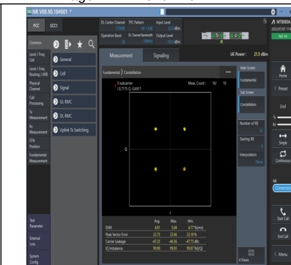
1-N26-814-824--15-10-M-6-CP-QPSK-Outer_Full-5 2@0-Ant1-see graph-PASS
