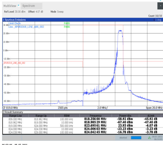
1-N26-814-824--15-5-H-2-DFT-PI2BPSK-Edge_1RB_Right-1@24-Ant1-PASS-see graph
