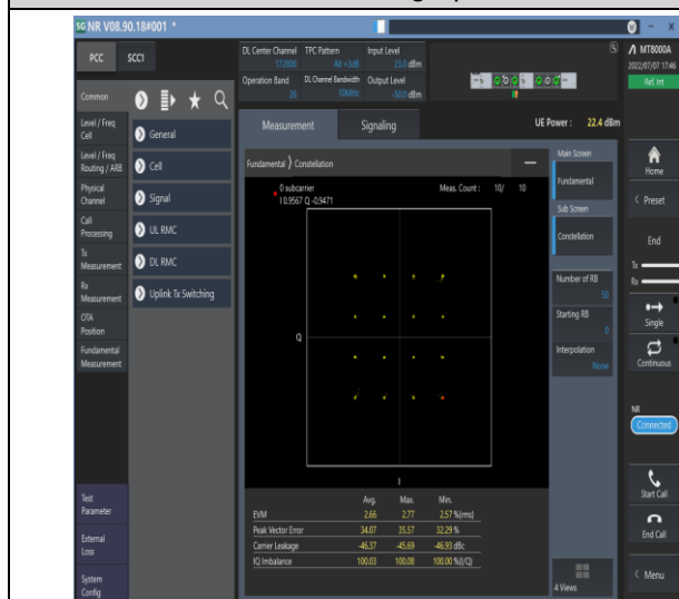
1-N26-814-824--15-10-M-3-DFT-16QAM-Out-0@0-Ant1-see graph-PASS
